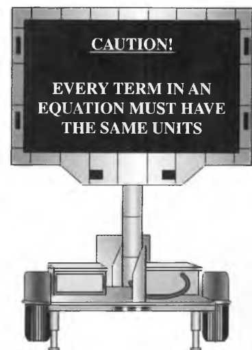
FIGURE 1–15 Always check the units in your calculations.
