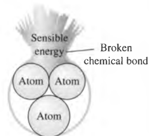
FIGURE 15-15 When the existing chemical bonds are destroyed and new ones are formed during a combustion process, usually a large amount of sensible energy is absorbed or released.
