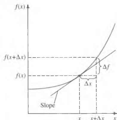
FIGURE 12-1 The derivative of a function at a specified point represents the slope of the function at that point.
