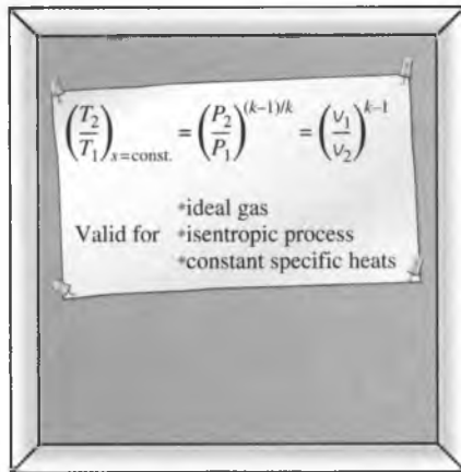
FIGURE 7-36 The isentropic relations of ideal gases are valid for the isentropic processes of ideal gases only.
