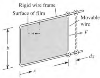
FIGURE 2-35 Stretching a liquid film with a movable wire.
