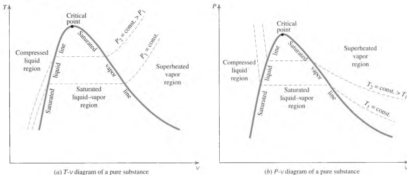
FIGURE 3-18 Property diagrams of a pure substance.
