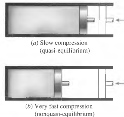
FIGURE 1–31 Quasi-equilibrium and nonquasi-equilibrium compression processes.
