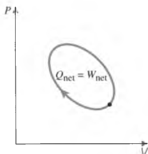
FIGURE 4-11 For a cycle \Delta E = 0 , thus Q = W .
