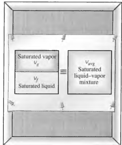
FIGURE 3–33 A two-phase system can be treated as a homogeneous mixture for convenience.
