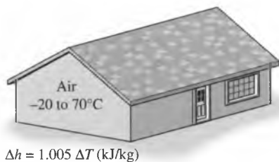
FIGURE 5-42 The error involved in \Delta h = c_p \Delta T , where c_p = 1.005 \text{ kJ/kg}\cdot^\circ\text{C} , is less than 0.5 percent for air in the temperature range -20 to 70^\circ\text{C} .
