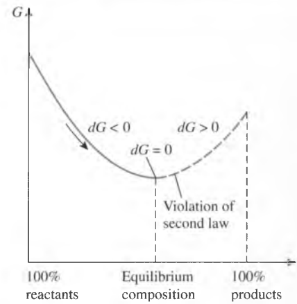
FIGURE 16-4 Criteria for chemical equilibrium for a fixed mass at a specified temperature and pressure.
