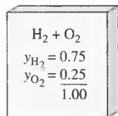
FIGURE 13-3 The sum of the mole fractions of a mixture is equal to 1.
