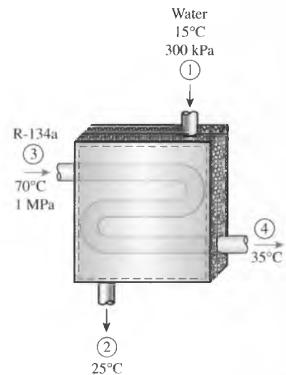
FIGURE 5-37 Schematic for Example 5-10.
