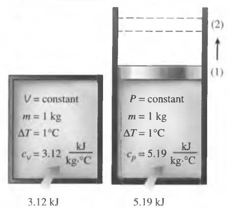
FIGURE 4-19 Constant-volume and constant-pressure specific heats c_v and c_p (values given are for helium gas).
