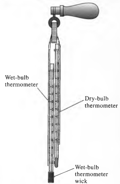
FIGURE 14–13 Sling psychrometer.
