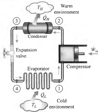
FIGURE 11-9 The vapor-compression refrigeration cycle considered in the second-law analysis.
