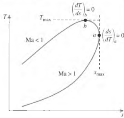
FIGURE 17-56 The T - s diagram of Rayleigh flow considered in Example 17-13.
