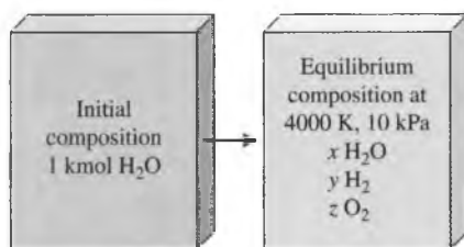
FIGURE 16-8 Schematic for Example 16-2.
