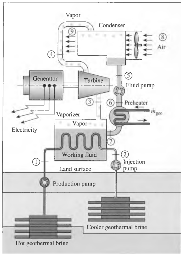
FIGURE P10-97 Schematic of a binary geothermal power plant.
