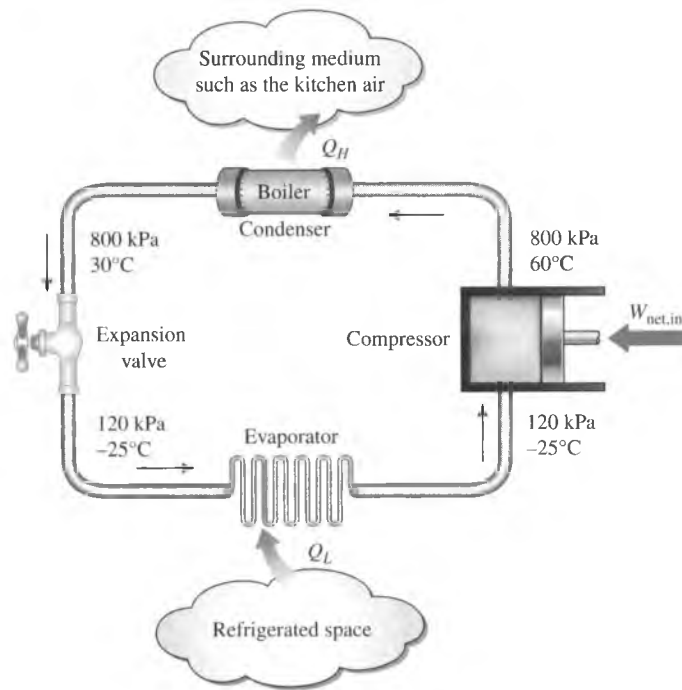
FIGURE 6-19 Basic components of a refrigeration system and typical operating conditions.
