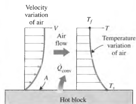
FIGURE 2-72 Heat transfer from a hot surface to air by convection.
