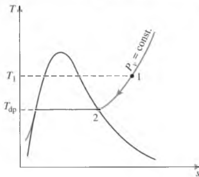
FIGURE 14-8 Constant-pressure cooling of moist air and the dew-point temperature on the T - s diagram of water.
