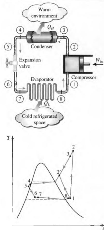
FIGURE 11-7 Schematic and T - s diagram for the actual vapor-compression refrigeration cycle.
