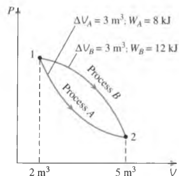
FIGURE 2–21 Properties are point functions; but heat and work are path functions (their magnitudes depend on the path followed).
