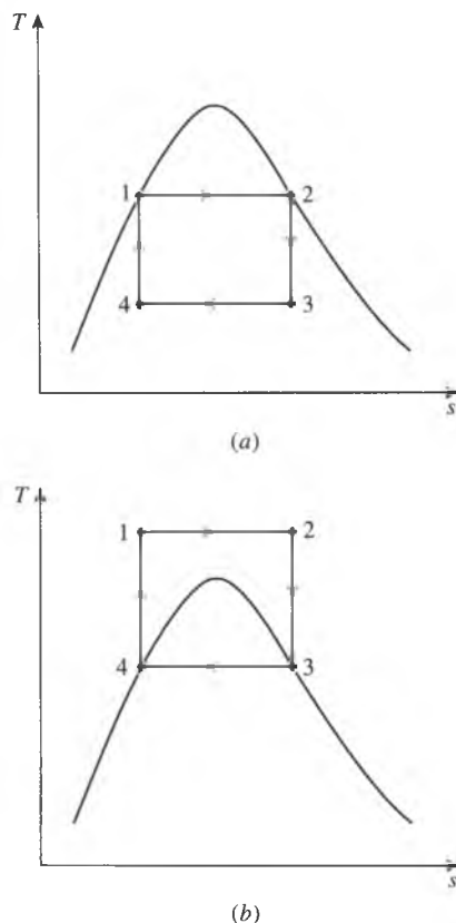
FIGURE 10-1 T - s diagram of two Carnot vapor cycles.
