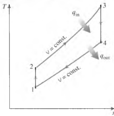
FIGURE 9-16 T-s diagram of the ideal Otto cycle.
