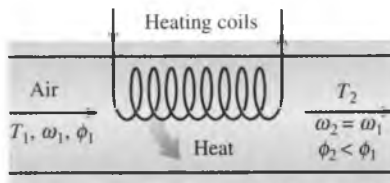
FIGURE 14-21 During simple heating, specific humidity remains constant, but relative humidity decreases.
