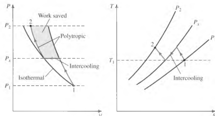
FIGURE 7-46 P - v and T - s diagrams for a two-stage steady-flow compression process.
