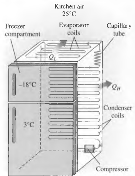
FIGURE 11-4 An ordinary household refrigerator.
