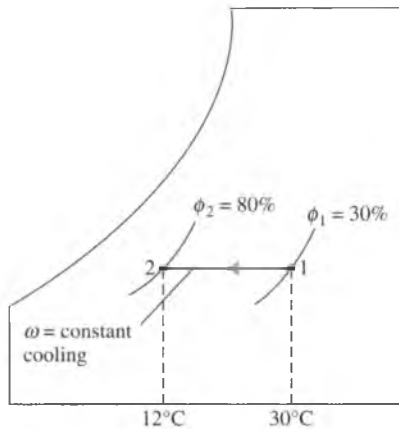
FIGURE 14-22 During simple cooling, specific humidity remains constant, but relative humidity increases.
