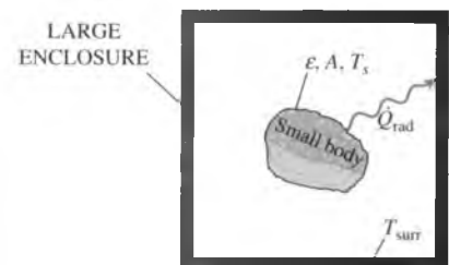
FIGURE 2-76 Radiation heat transfer between a body and the inner surfaces of a much larger enclosure that completely surrounds it.
