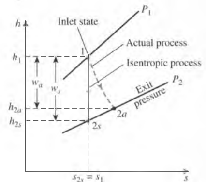
FIGURE 7-49 The h - s diagram for the actual and isentropic processes of an adiabatic turbine.
