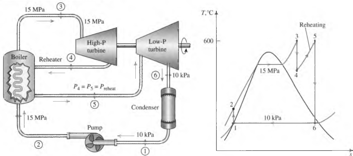
FIGURE 10-13 Schematic and T - s diagram for Example 10-4.
