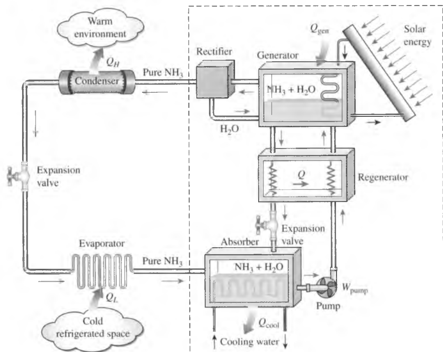
FIGURE 11-23 Ammonia absorption refrigeration cycle.
