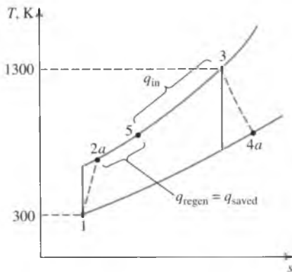
FIGURE 9-41 T-s diagram of the regenerative Brayton cycle described in Example 9-7.
