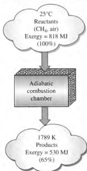
FIGURE 15–35 The availability of methane decreases by 35 percent as a result of irreversible combustion process.
