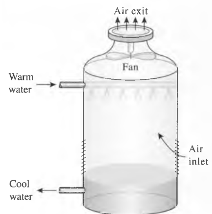
FIGURE 14–31 An induced-draft counterflow cooling tower.
