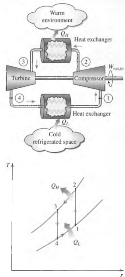
FIGURE 11-18 Simple gas refrigeration cycle.
