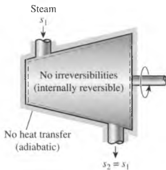
FIGURE 7-14 During an internally reversible, adiabatic (isentropic) process, the entropy remains constant.
