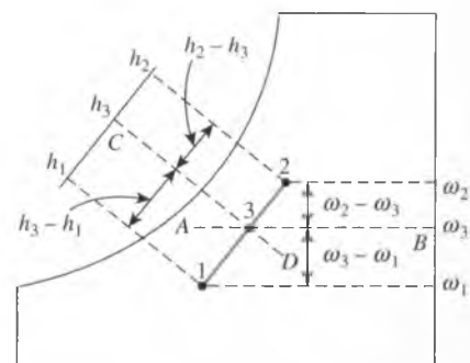
FIGURE 14-29 When two airstreams at states 1 and 2 are mixed adiabatically, the state of the mixture lies on the straight line connecting the two states.
