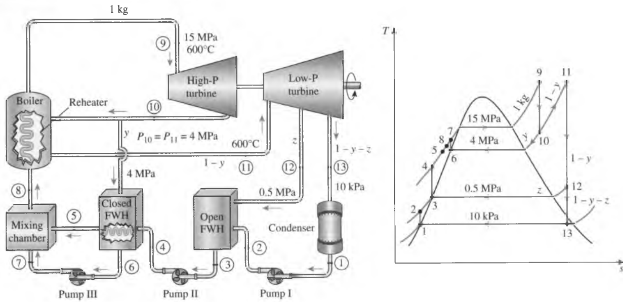
FIGURE 10-19 Schematic and T - s diagram for Example 10-6.
