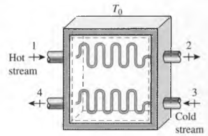
FIGURE 8-44 A heat exchanger with two unmixed fluid streams.
