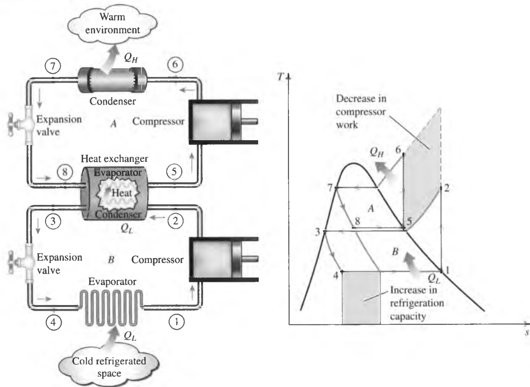
FIGURE 11-12 A two-stage cascade refrigeration system with the same refrigerant in both stages.
