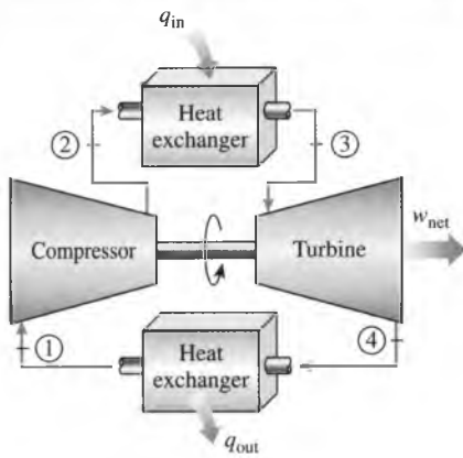
FIGURE 9-30 A closed-cycle gas-turbine engine.
