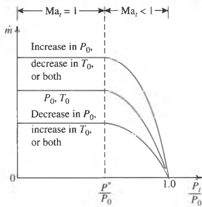
FIGURE 17-22 The variation of the mass flow rate through a nozzle with inlet stagnation properties.
