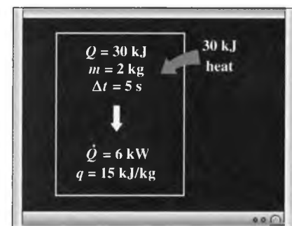
FIGURE 2-17 The relationships among q , Q , and \dot{Q} .
