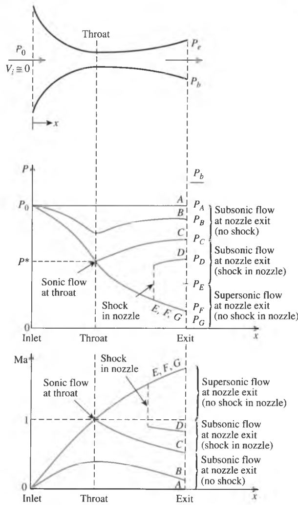
FIGURE 17-27 The effects of back pressure on the flow through a converging–diverging nozzle.
