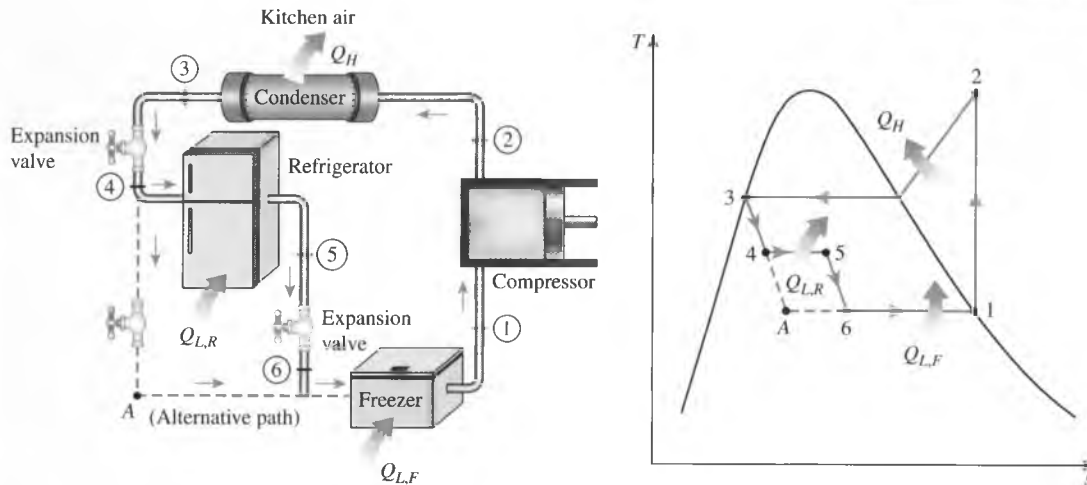
FIGURE 11–16 Schematic and T - s diagram for a refrigerator–freezer unit with one compressor.
