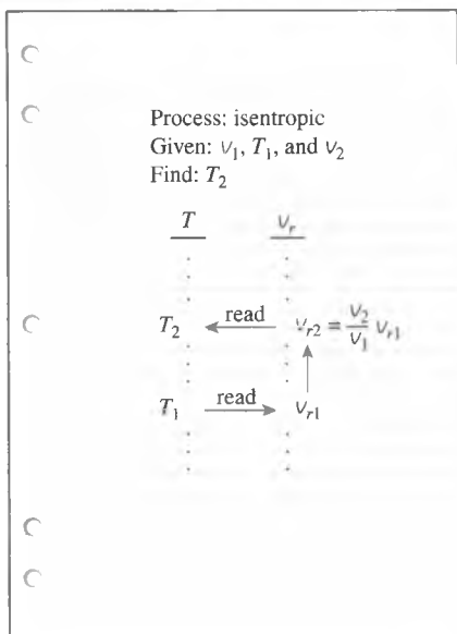
FIGURE 7-39 The use of v_r data for calculating the final temperature during an isentropic process (Example 7-10).
