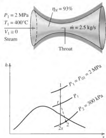
FIGURE 17-62 Schematic and h - s diagram for Example 17-16.
