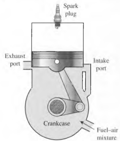
FIGURE 9–14 Schematic of a two-stroke reciprocating engine.
