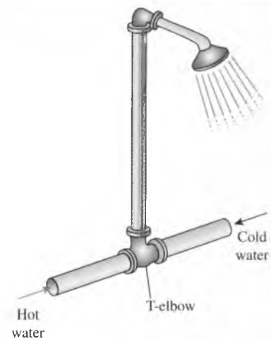
FIGURE 5–32 The T-elbow of an ordinary shower serves as the mixing chamber for the hot- and the cold-water streams.
