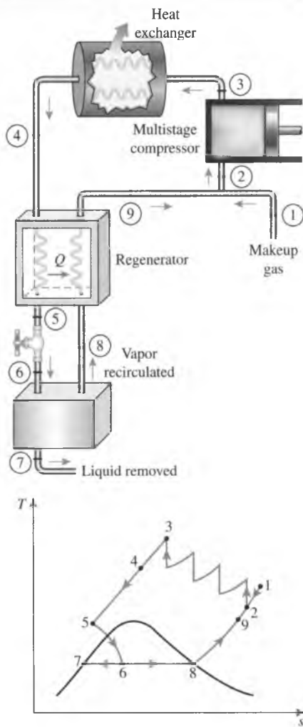
FIGURE 11-17 Linde-Hampson system for liquefying gases.
