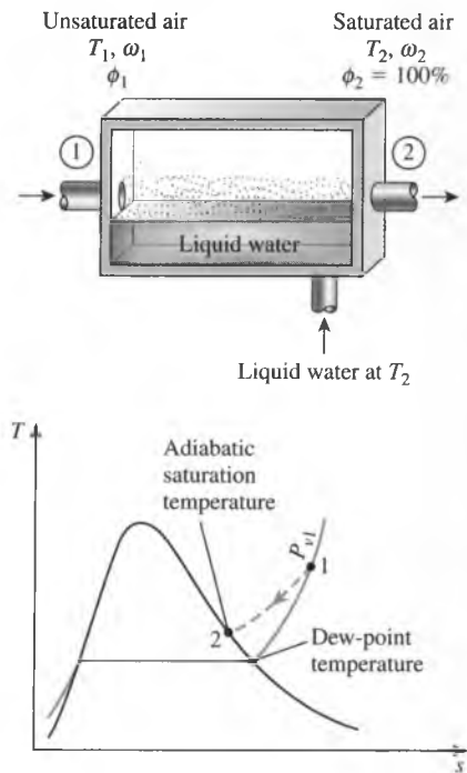
FIGURE 14-11 The adiabatic saturation process and its representation on a T - s diagram of water.
