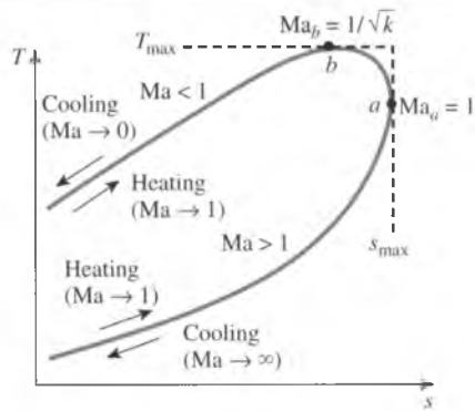
FIGURE 17-54 T - s diagram for flow in a constant-area duct with heat transfer and negligible friction (Rayleigh flow).
