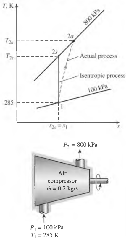
FIGURE 7-53 Schematic and T - s diagram for Example 7-15.
