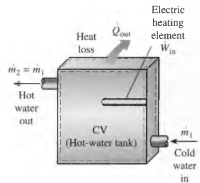
FIGURE 5-20 A water heater in steady operation.
