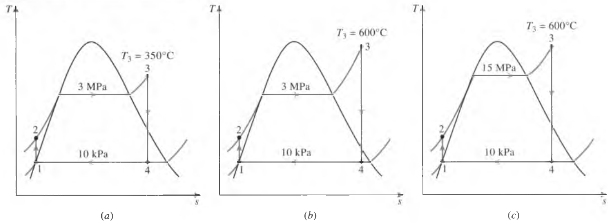
FIGURE 10-10 T - s diagrams of the three cycles discussed in Example 10-3.
