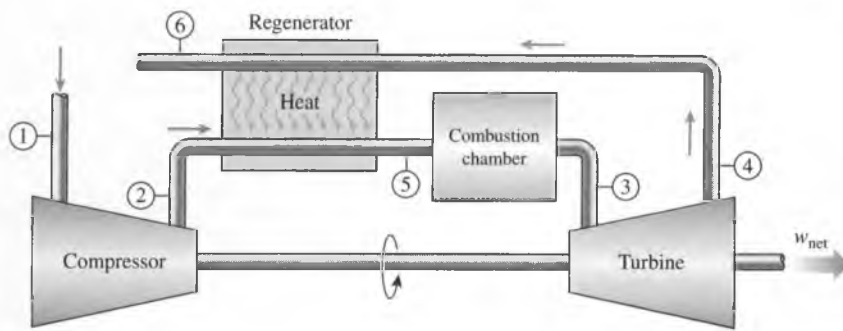
FIGURE 9-38 A gas-turbine engine with regenerator.
