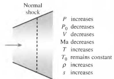
FIGURE 17-32 Variation of flow properties across a normal shock.
