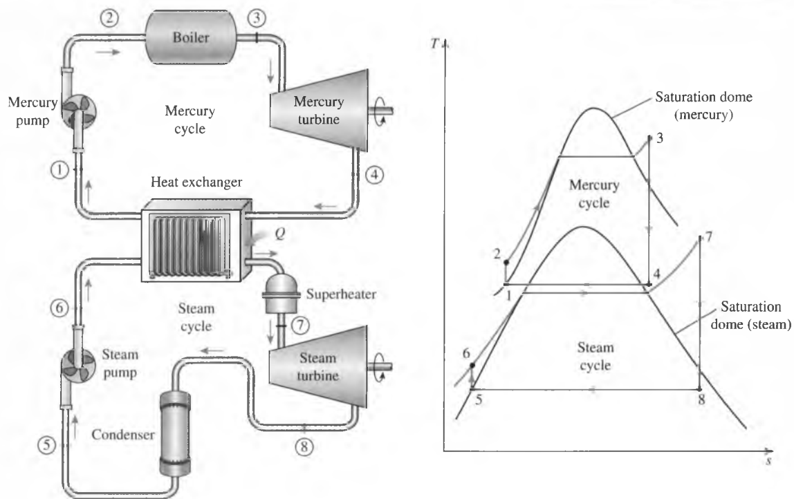
FIGURE 10-27 Mercury–water binary vapor cycle.
