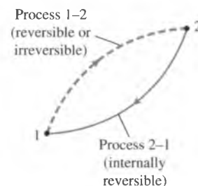
FIGURE 7-5 A cycle composed of a reversible and an irreversible process.
