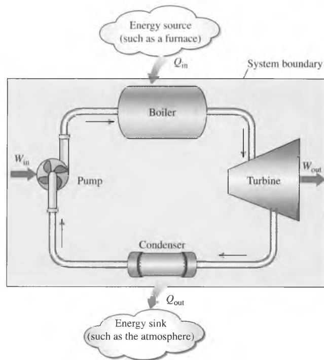
FIGURE 6-10 Schematic of a steam power plant.
