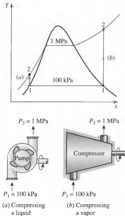
FIGURE 7-43 Schematic and T-s diagram for Example 7-12.
