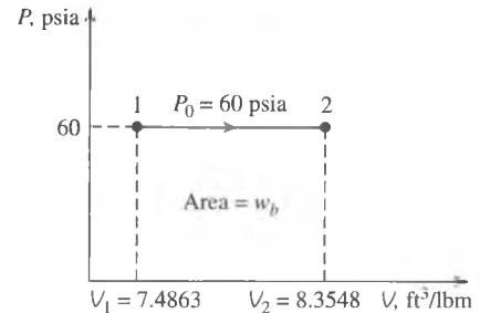
FIGURE 4-7 Schematic and P - v diagram for Example 4-2.
