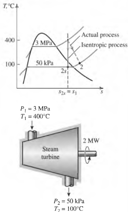
FIGURE 7-50 Schematic and T - s diagram for Example 7-14.
