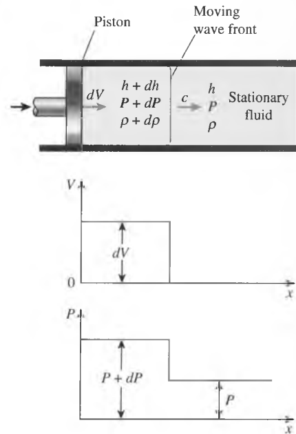
FIGURE 17-7 Propagation of a small pressure wave along a duct.
