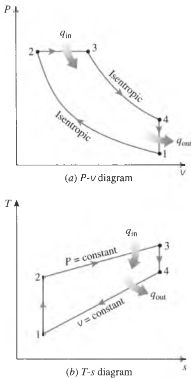
FIGURE 9-21 T - s and P - v diagrams for the ideal Diesel cycle.
