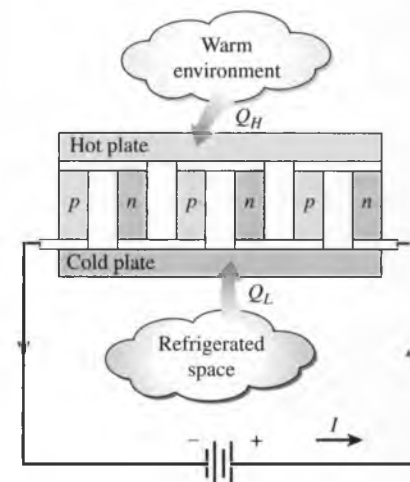
FIGURE 11–30 A thermoelectric refrigerator.
