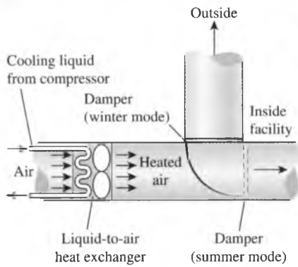
FIGURE 7-80 Waste heat from a compressor can be used to heat a building in winter.
