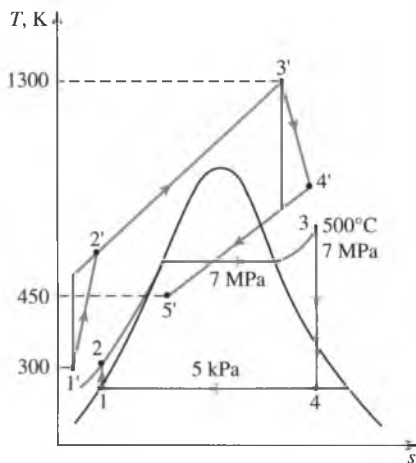
FIGURE 10–26 T - s diagram of the gas–steam combined cycle described in Example 10–9.
