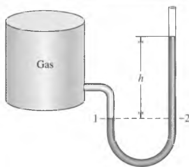
FIGURE 1-49 The basic manometer.
