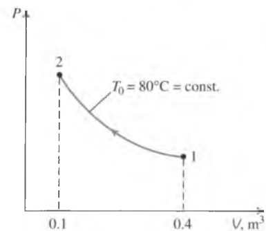
FIGURE 4-8 Schematic and P - V diagram for Example 4-3.
