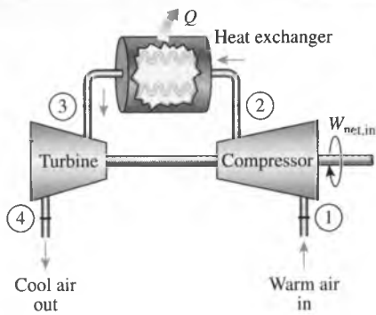
FIGURE 11-20 An open-cycle aircraft cooling system.
