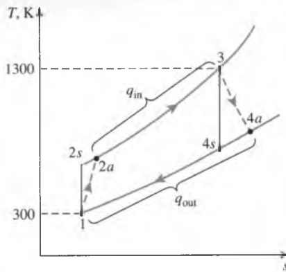
FIGURE 9-37 T-s diagram of the gas-turbine cycle discussed in Example 9-6.
