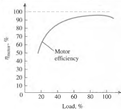
FIGURE 7-77 The efficiency of an electric motor decreases at part load.
