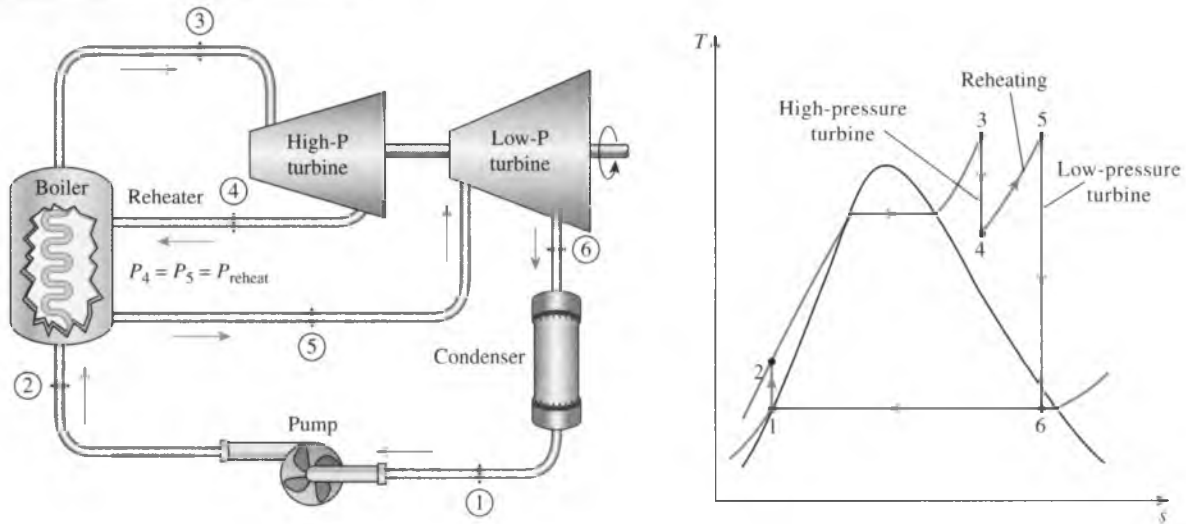
FIGURE 10-11 The ideal reheat Rankine cycle.
