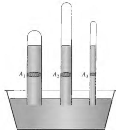
FIGURE 1-56 The length or the cross-sectional area of the tube has no effect on the height of the fluid column of a barometer, provided that the tube diameter is large enough to avoid surface tension (capillary) effects.
