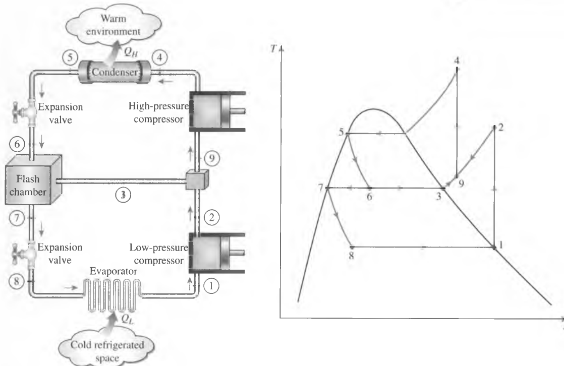
FIGURE 11-14 A two-stage compression refrigeration system with a flash chamber.
