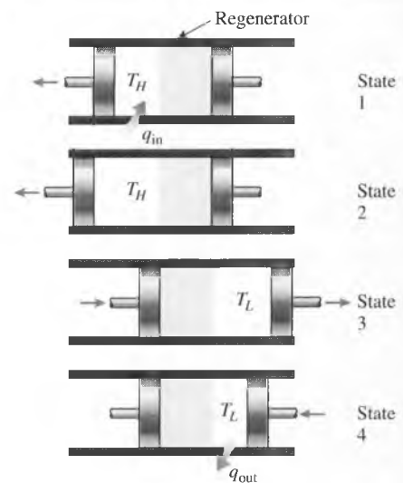
FIGURE 9–27 The execution of the Stirling cycle.
