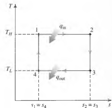
FIGURE 9-8 T - s diagram for Example 9-1.
