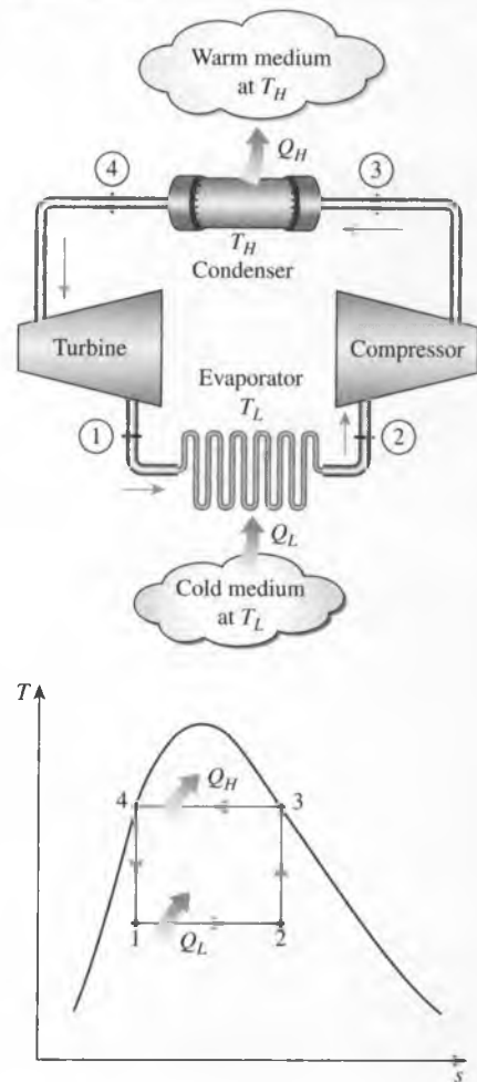
FIGURE 11-2 Schematic of a Carnot refrigerator and T - s diagram of the reversed Carnot cycle.
