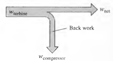
FIGURE 9–34 The fraction of the turbine work used to drive the compressor is called the back work ratio.
