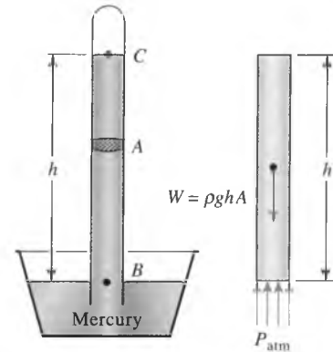
FIGURE 1-55 The basic barometer.
