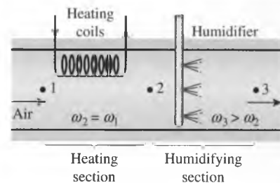
FIGURE 14-23 Heating with humidification.
