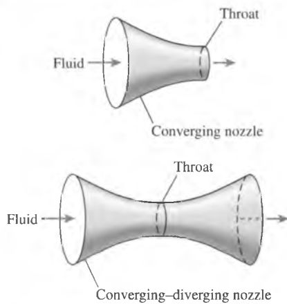
FIGURE 17-14 The cross section of a nozzle at the smallest flow area is called the throat .
