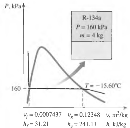
FIGURE 3-37 Schematic and P - v diagram for Example 3-5.
