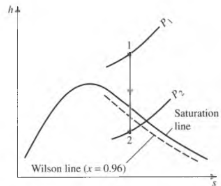
FIGURE 17-61 The h - s diagram for the isentropic expansion of steam in a nozzle.
