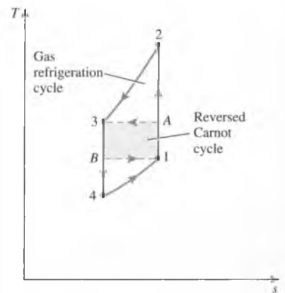
FIGURE 11-19 A reserved Carnot cycle produces more refrigeration (area under B1 ) with less work input (area 1A3B ).
