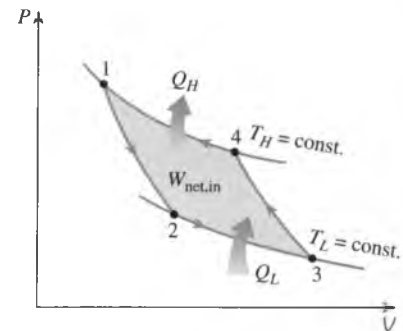
FIGURE 6-39 P - V diagram of the reversed Carnot cycle.
