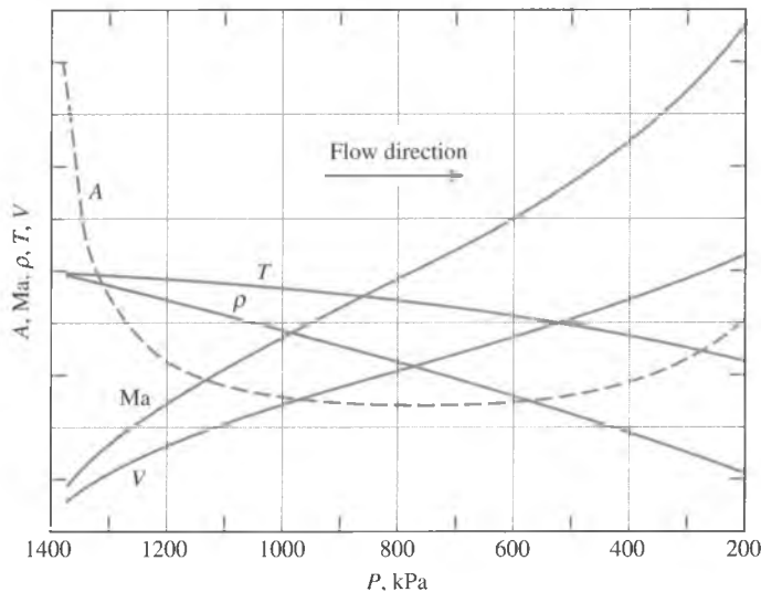
FIGURE 17-13 Variation of normalized fluid properties and cross-sectional area along a duct as the pressure drops from 1400 to 200 kPa.
