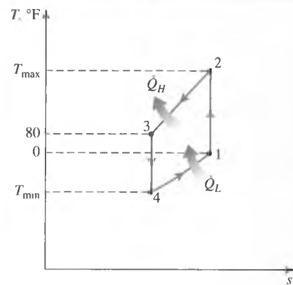
FIGURE 11-22 T-s diagram of the ideal-gas refrigeration cycle described in Example 11-6.
