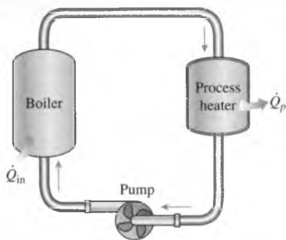
FIGURE 10-21 A simple process-heating plant.
