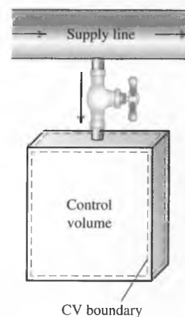
FIGURE 5-43 Charging of a rigid tank from a supply line is an unsteady-flow process since it involves changes within the control volume.
