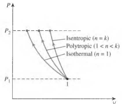
FIGURE 7-45 P - v diagrams of isentropic, polytropic, and isothermal compression processes between the same pressure limits.
