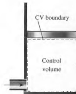
FIGURE 5-44 The shape and size of a control volume may change during an unsteady-flow process.
