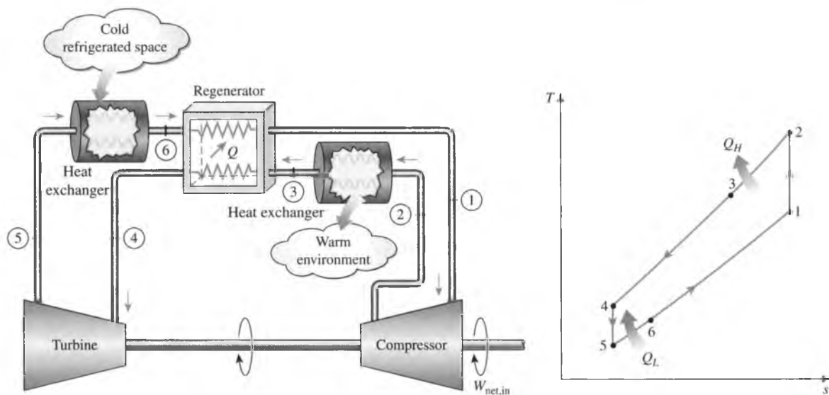
FIGURE 11-21 Gas refrigeration cycle with regeneration.
