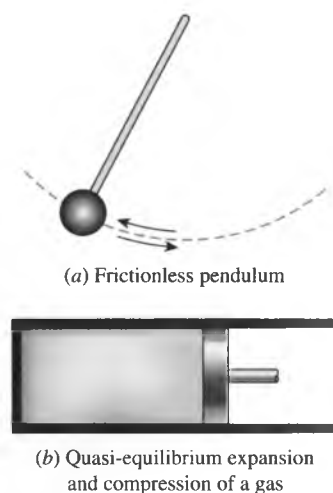
FIGURE 6-30 Two familiar reversible processes.
