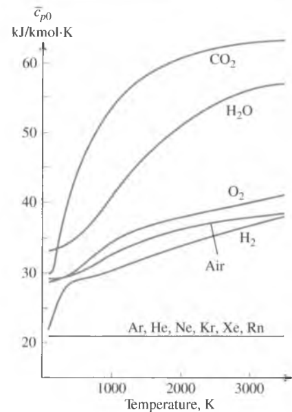
FIGURE 4-24 Ideal-gas constant-pressure specific heats for some gases (see Table A-2c for c_p equations).
