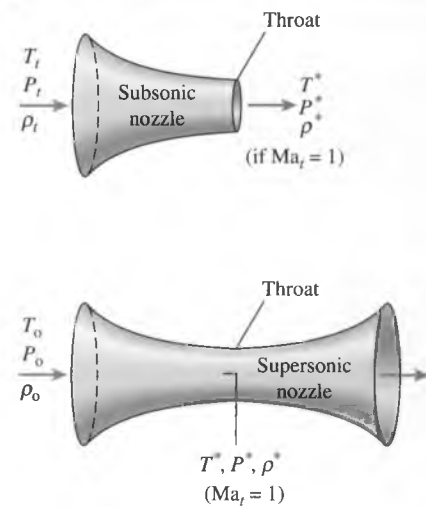
FIGURE 17-18 When \text{Ma}_t = 1 , the properties at the nozzle throat become the critical properties.
