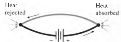
FIGURE 11–29 When a current is passed through the junction of two dissimilar materials, the junction is cooled.
