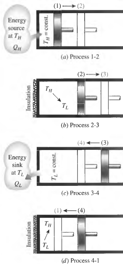
FIGURE 6-37 Execution of the Carnot cycle in a closed system.
