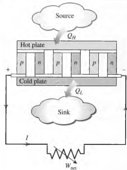
FIGURE 11–28 A thermoelectric power generator.
