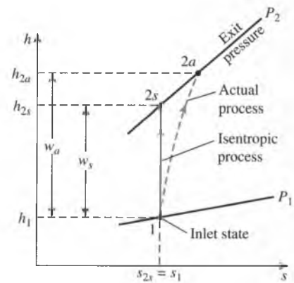
FIGURE 7-51 The h - s diagram of the actual and isentropic processes of an adiabatic compressor.
