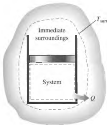
FIGURE 7-62 Entropy generation outside system boundaries can be accounted for by writing an entropy balance on an extended system that includes the system and its immediate surroundings.
