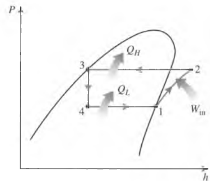
FIGURE 11-5 The P - h diagram of an ideal vapor-compression refrigeration cycle.
