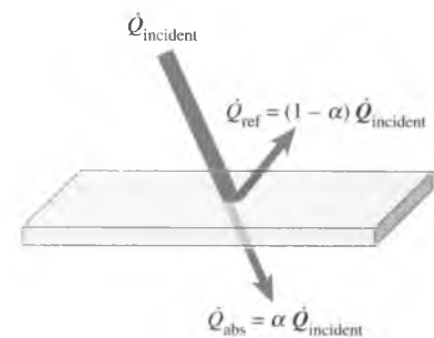
FIGURE 2-75 The absorption of radiation incident on an opaque surface of absorptivity \alpha .
