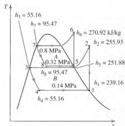
FIGURE 11–13 T - s diagram of the cascade refrigeration cycle described in Example 11–4.
