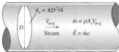
FIGURE 2-4 Mass and energy flow rates associated with the flow of steam in a pipe of inner diameter D with an average velocity of V_{avg} .
