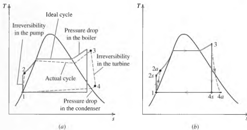
FIGURE 10-4 (a) Deviation of actual vapor power cycle from the ideal Rankine cycle. (b) The effect of pump and turbine irreversibilities on the ideal Rankine cycle.
