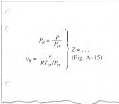
FIGURE 3-52 The compressibility factor can also be determined from a knowledge of P_R and v_R .
