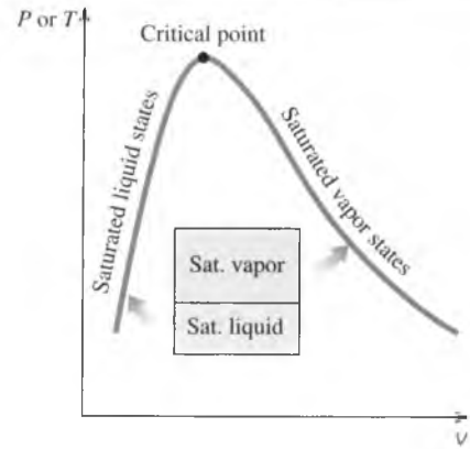
FIGURE 3–32 The relative amounts of liquid and vapor phases in a saturated mixture are specified by the quality x .
