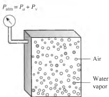
FIGURE 3-59 Atmospheric pressure is the sum of the dry air pressure P_a and the vapor pressure P_v .
