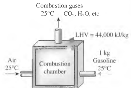
FIGURE 2-56 The definition of the heating value of gasoline.
