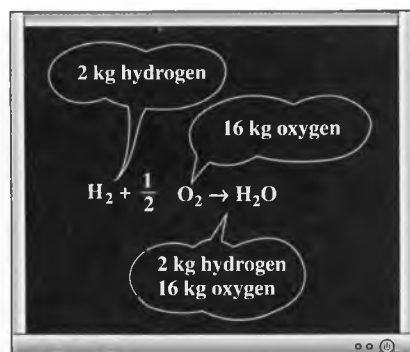
FIGURE 15-5 The mass (and number of atoms) of each element is conserved during a chemical reaction.
