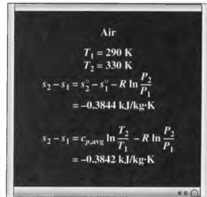
FIGURE 7-35 For small temperature differences, the exact and approximate relations for entropy changes of ideal gases give almost identical results.
