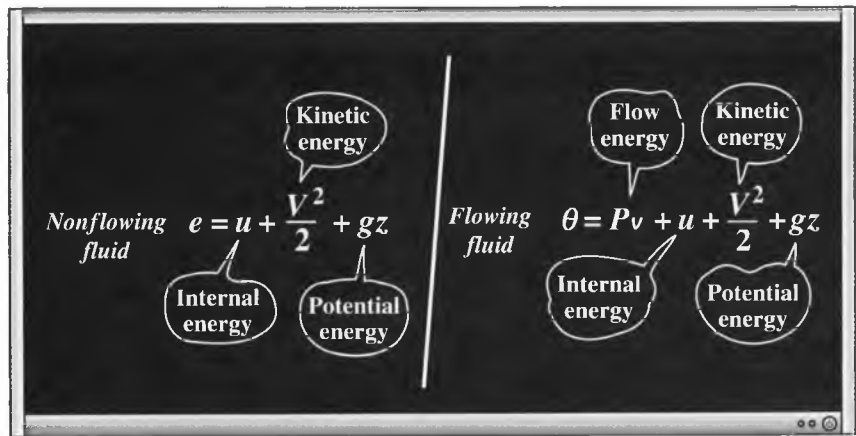
FIGURE 5-14 The total energy consists of three parts for a nonflowing fluid and four parts for a flowing fluid.
