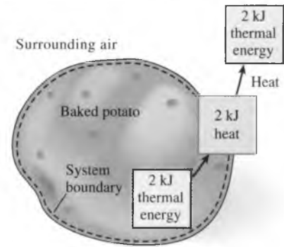
FIGURE 2-15 Energy is recognized as heat transfer only as it crosses the system boundary.
