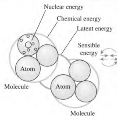
FIGURE 15-14 The microscopic form of energy of a substance consists of sensible, latent, chemical, and nuclear energies.
