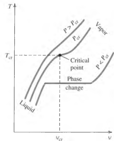
FIGURE 3-17 At supercritical pressures ( P > P_{cr} ), there is no distinct phase-change (boiling) process.
