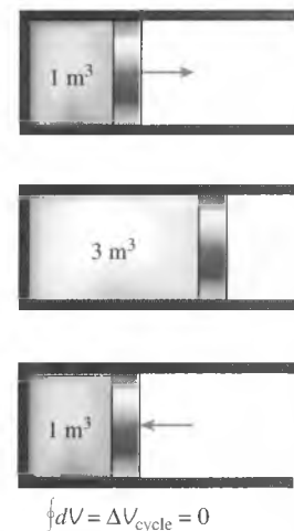
FIGURE 7-2 The net change in volume (a property) during a cycle is always zero.
