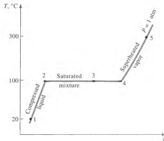
FIGURE 3-11 T - v diagram for the heating process of water at constant pressure.
