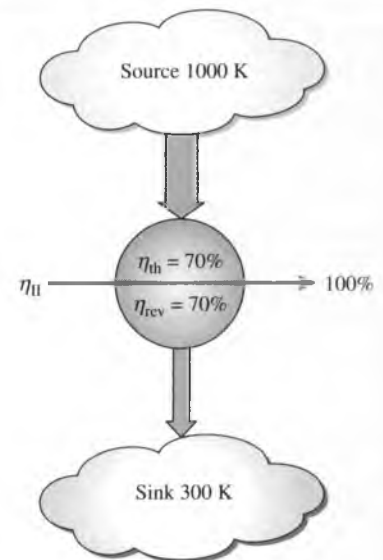
FIGURE 8-17 Second-law efficiency of all reversible devices is 100 percent.
