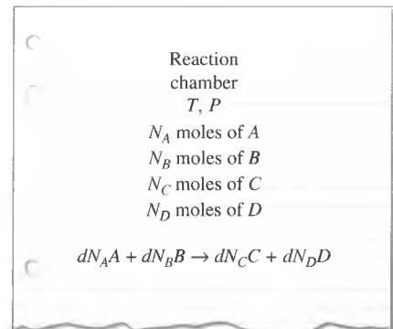
FIGURE 16-5 An infinitesimal reaction in a chamber at constant temperature and pressure.
