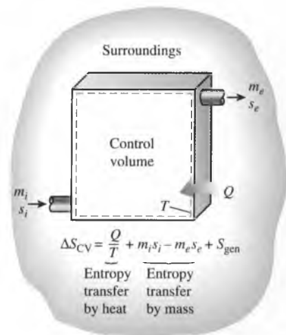
FIGURE 7-63 The entropy of a control volume changes as a result of mass flow as well as heat transfer.
