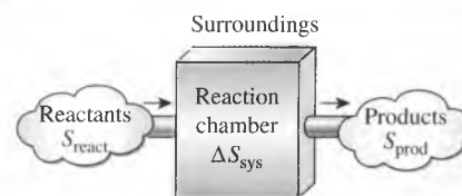
FIGURE 15–28 The entropy change associated with a chemical relation.
