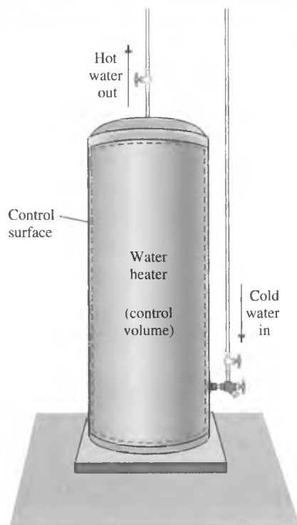
FIGURE 1-23 An open system (a control volume) with one inlet and one exit.
