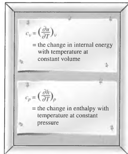
FIGURE 4-20 Formal definitions of c_v and c_p .
