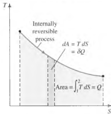
FIGURE 7-16 On a T - S diagram, the area under the process curve represents the heat transfer for internally reversible processes.
