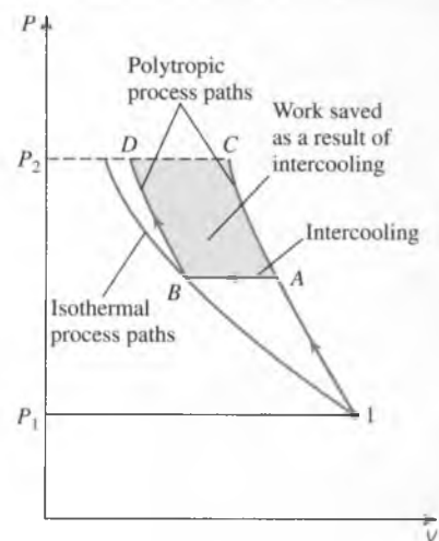
FIGURE 9-42 Comparison of work inputs to a single-stage compressor (1AC) and a two-stage compressor with intercooling (1ABD).
