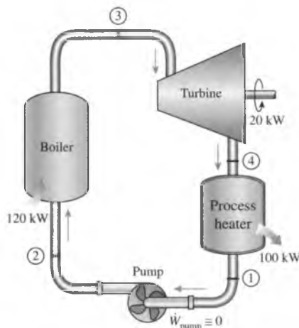
FIGURE 10-22 An ideal cogeneration plant.
