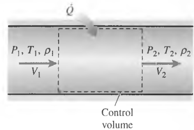
FIGURE 17–53 Control volume for flow in a constant-area duct with heat transfer and negligible friction.
