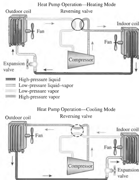
FIGURE 11-11 A heat pump can be used to heat a house in winter and to cool it in summer.
