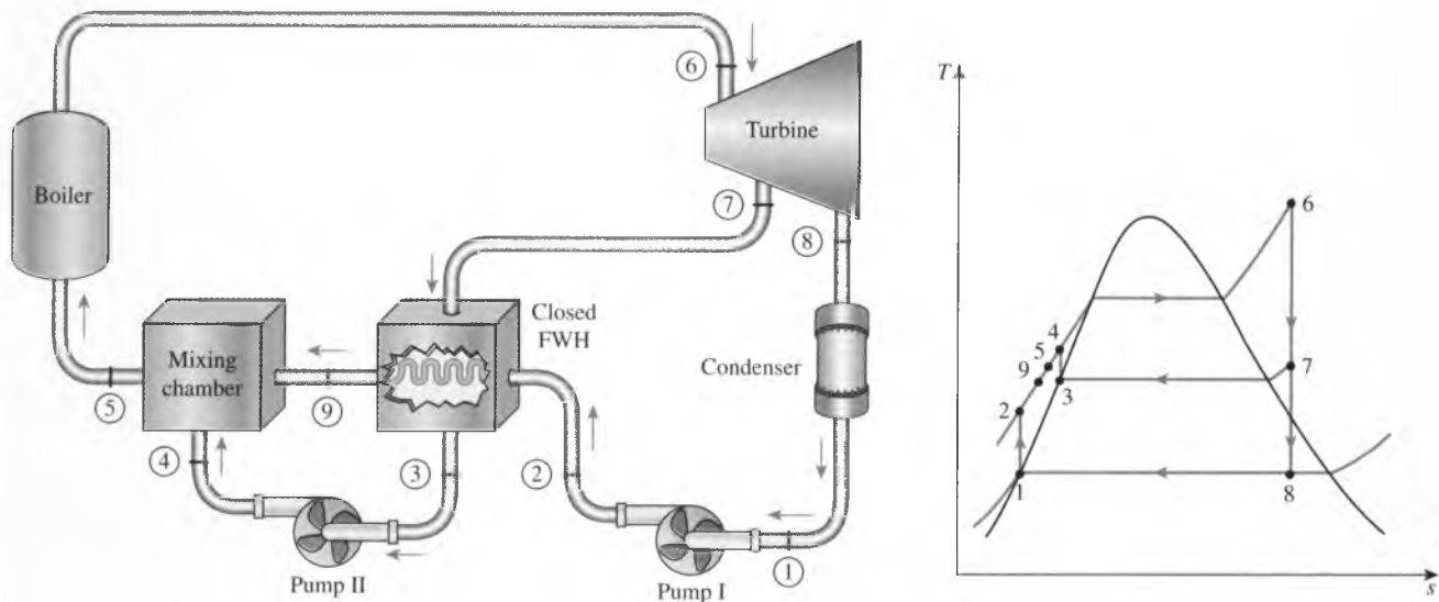
FIGURE 10–16 The ideal regenerative Rankine cycle with a closed feedwater heater.
