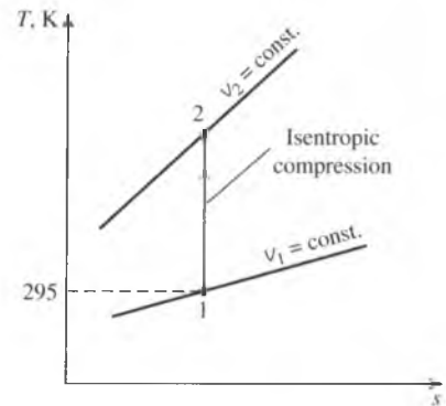
FIGURE 7-37 The use of P_r data for calculating the final temperature during an isentropic process.
