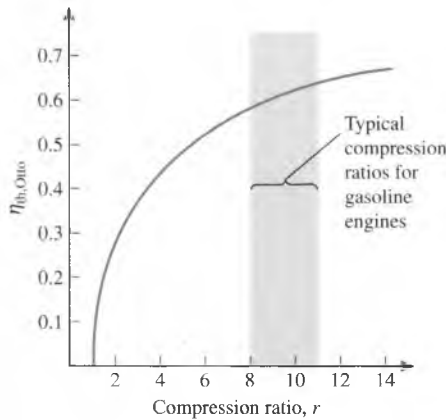
FIGURE 9-17 Thermal efficiency of the ideal Otto cycle as a function of compression ratio ( k = 1.4 ).
