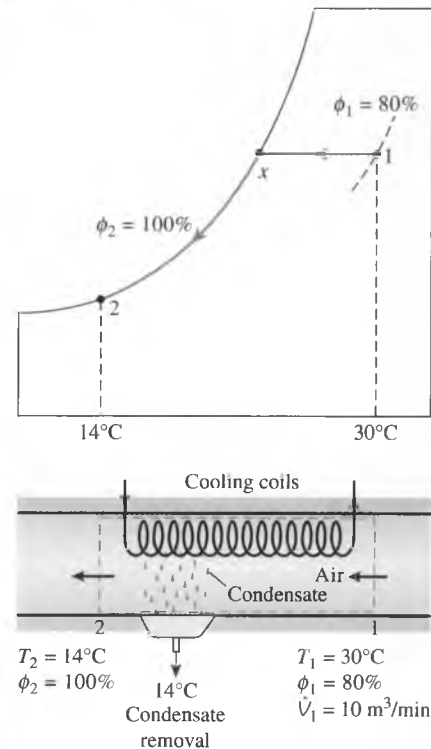
FIGURE 14–25 Schematic and psychrometric chart for Example 14–6.
