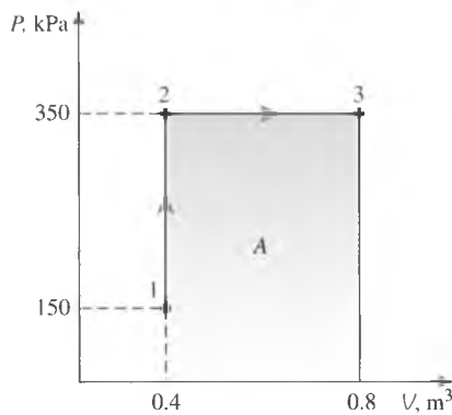
FIGURE 4-32 Schematic and P - V diagram for Example 4-10.
