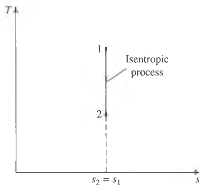
FIGURE 7-17 The isentropic process appears as a vertical line segment on a T - s diagram.
