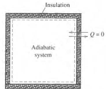
FIGURE 2-16 During an adiabatic process, a system exchanges no heat with its surroundings.
