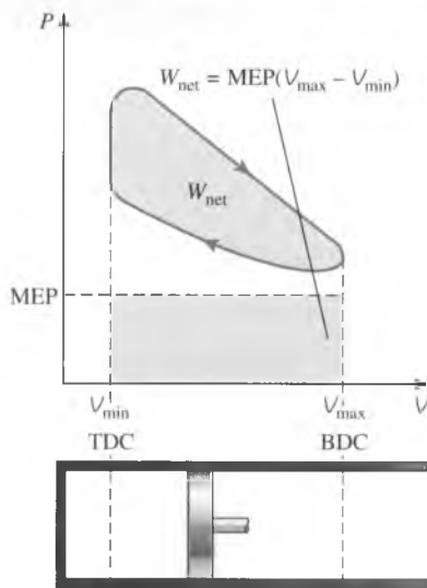
FIGURE 9-12 The net work output of a cycle is equivalent to the product of the mean effective pressure and the displacement volume.
