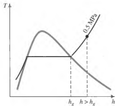
FIGURE 3–39 At a specified P , superheated vapor exists at a higher h than the saturated vapor (Example 3–7).
