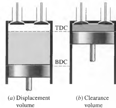
FIGURE 9–11 Displacement and clearance volumes of a reciprocating engine.
