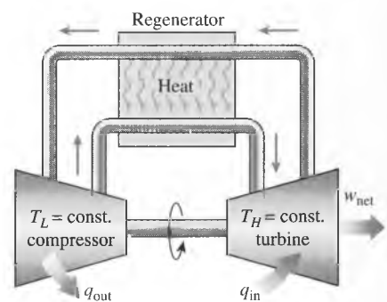
FIGURE 9–28 A steady-flow Ericsson engine.
