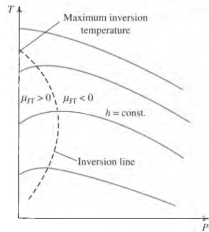
FIGURE 12-14 Constant-enthalpy lines of a substance on a T - P diagram.
