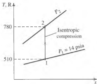
FIGURE 7-39 The use of v_r data for calculating the final temperature during an isentropic process (Example 7-10).
