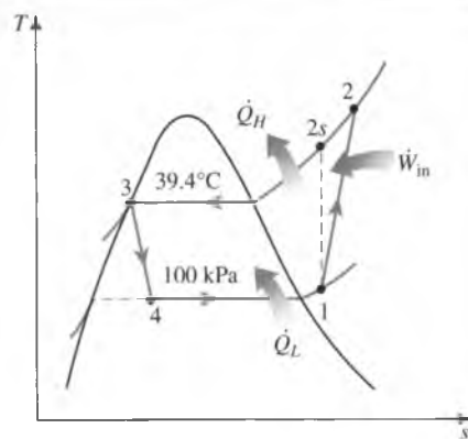
FIGURE 11-10 Temperature-entropy diagram of the vapor-compression refrigeration cycle considered in Example 11-3.
