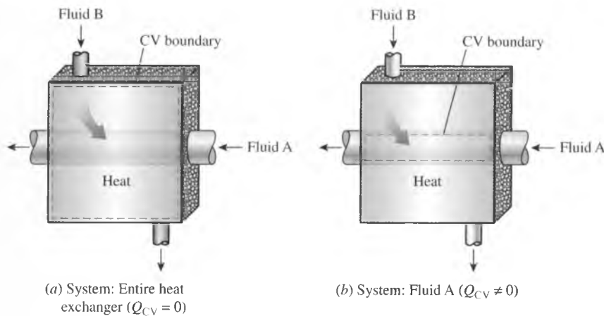
FIGURE 5-36 The heat transfer associated with a heat exchanger may be zero or nonzero depending on how the control volume is selected.
