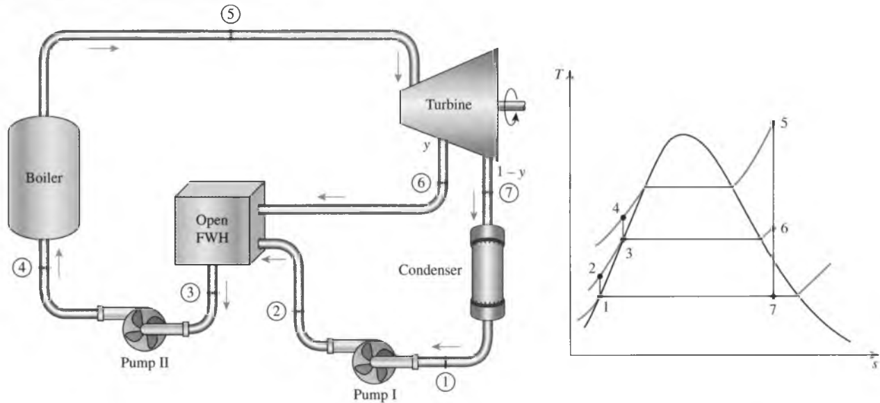
FIGURE 10-15 The ideal regenerative Rankine cycle with an open feedwater heater.
