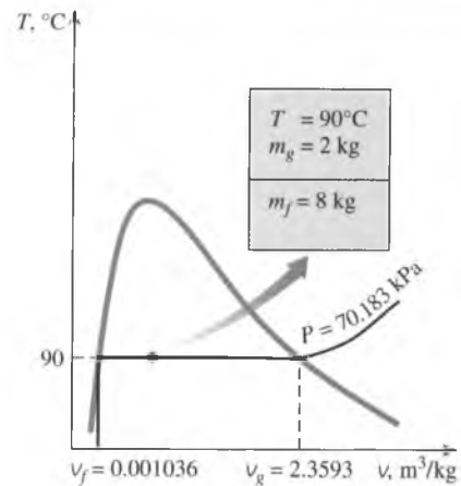
FIGURE 3-36 Schematic and T - v diagram for Example 3-4.
