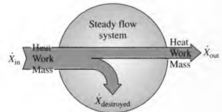
FIGURE 8–43 The exergy transfer to a steady-flow system is equal to the exergy transfer from it plus the exergy destruction within the system.
