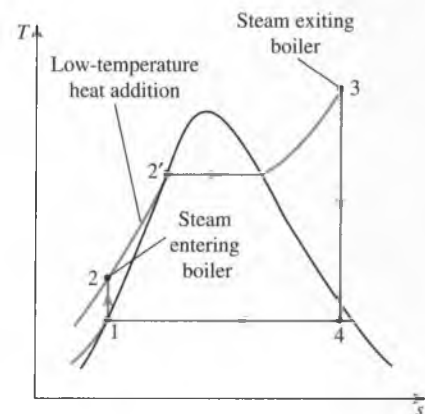
FIGURE 10–14 The first part of the heat-addition process in the boiler takes place at relatively low temperatures.
