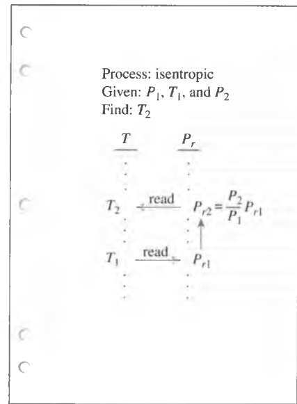
FIGURE 7-37 The use of P_r data for calculating the final temperature during an isentropic process.
