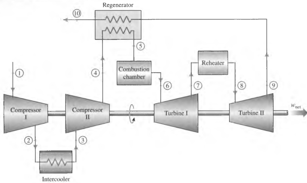
FIGURE 9-43 A gas-turbine engine with two-stage compression with intercooling, two-stage expansion with reheating, and regeneration.
