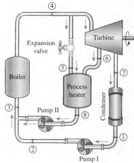
FIGURE 10-23 A cogeneration plant with adjustable loads.
