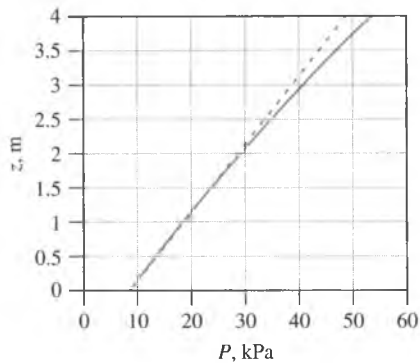
FIGURE 1-60 The variation of gage pressure with depth in the gradient zone of the solar pond.
