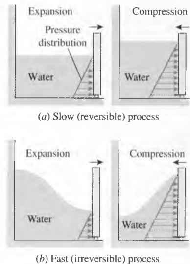
FIGURE 6–31 Reversible processes deliver the most and consume the least work.
