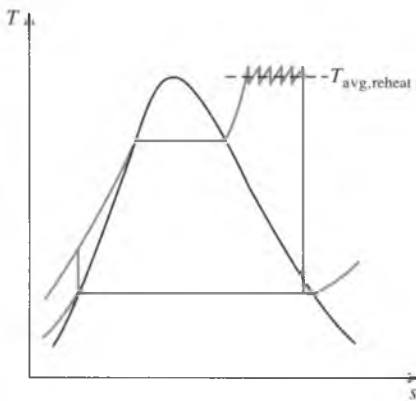
FIGURE 10-12 The average temperature at which heat is transferred during reheating increases as the number of reheat stages is increased.
