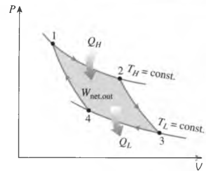
FIGURE 6-38 P - V diagram of the Carnot cycle.
