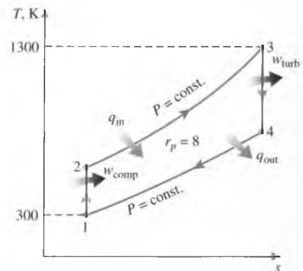
FIGURE 9-35 T - s diagram for the Brayton cycle discussed in Example 9-5.
