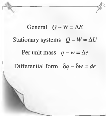
FIGURE 4-12 Various forms of the first-law relation for closed systems.
