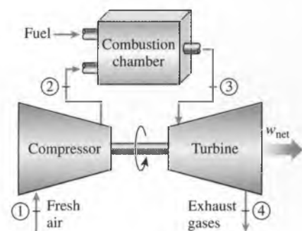
FIGURE 9-29 An open-cycle gas-turbine engine.
