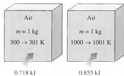
FIGURE 4-21 The specific heat of a substance changes with temperature.
