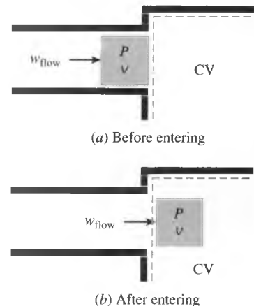
FIGURE 5-13 Flow work is the energy needed to push a fluid into or out of a control volume, and it is equal to Pv .
