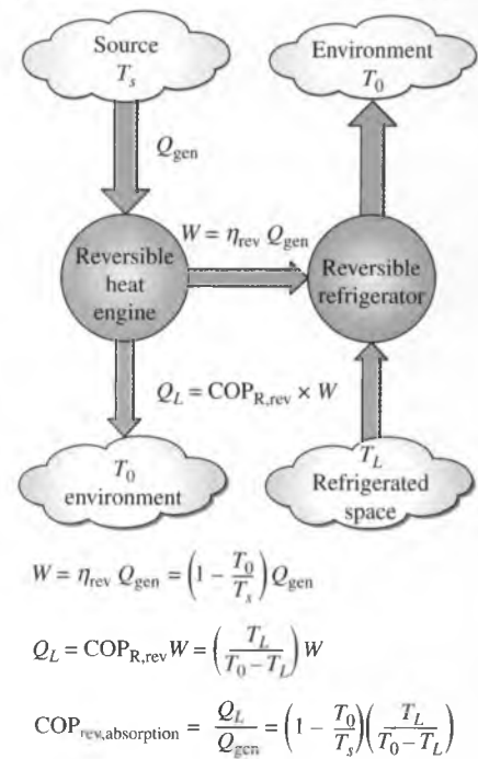
FIGURE 11-24 Determining the maximum COP of an absorption refrigeration system.
