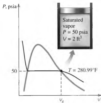
FIGURE 3-30 Schematic and P - v diagram for Example 3-2.
