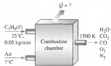
FIGURE 15-23 Schematic for Example 15-6.
