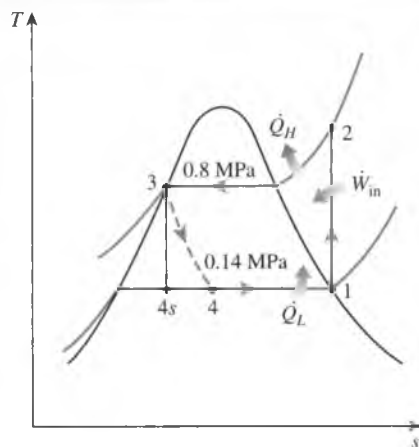
FIGURE 11-6 T-s diagram of the ideal vapor-compression refrigeration cycle described in Example 11-1.
