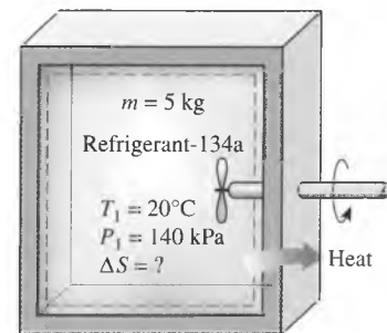
FIGURE 7-12 Schematic and T - s diagram for Example 7-3.
