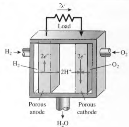
FIGURE 15–36 The operation of a hydrogen–oxygen fuel cell.
