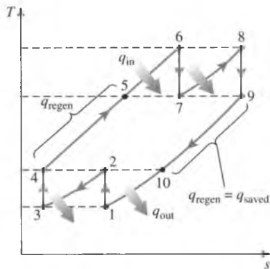
FIGURE 9-44 T-s diagram of an ideal gas-turbine cycle with intercooling, reheating, and regeneration.
