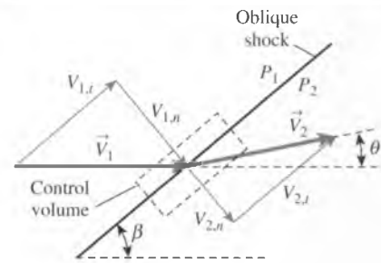
FIGURE 17-40 Velocity vectors through an oblique shock of shock angle \beta and deflection angle \theta .
