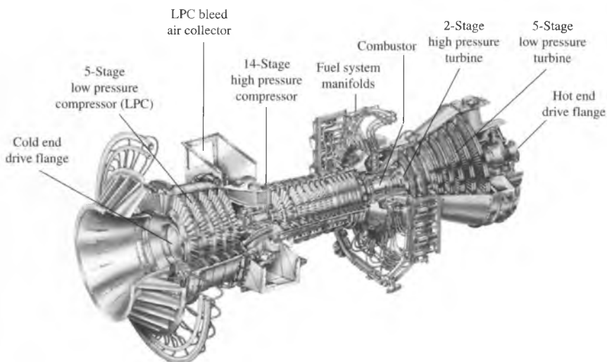
FIGURE 5–24 A modern land-based gas turbine used for electric power production. This is a General Electric LM5000 turbine. It has a length of 6.2 \text{m} , it weighs 12.5 tons, and produces 55.2 \text{MW} at 3600 \text{rpm} with steam injection. Courtesy of GE Power Systems.
