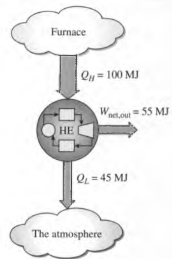
FIGURE 6–14 Even the most efficient heat engines reject almost one-half of the energy they receive as waste heat.
