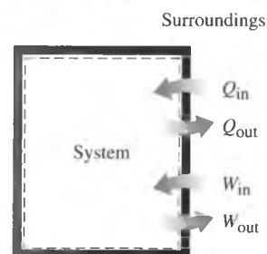
FIGURE 2–20 Specifying the directions of heat and work.
