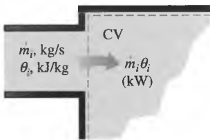
FIGURE 5-15 The product \dot{m}_e \theta_e is the energy transported into control volume by mass per unit time.
