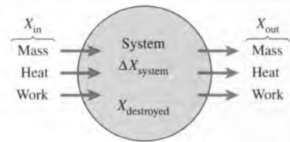
FIGURE 8-32 Mechanisms of exergy transfer.
