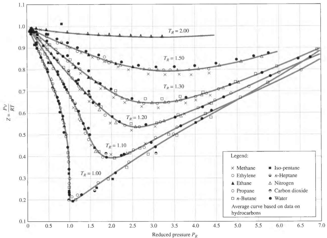
FIGURE 3-49 Comparison of Z factors for various gases.
