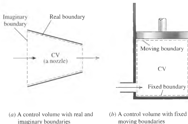
FIGURE 1-22 A control volume can involve fixed, moving, real, and imaginary boundaries.
