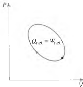
FIGURE 2-48 For a cycle \Delta E = 0 , thus Q = W .
