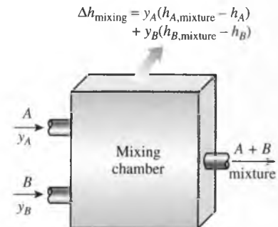
FIGURE 13-19 The amount of heat released or absorbed during a mixing process is called the enthalpy (or heat) of mixing, which is zero for ideal solutions.
