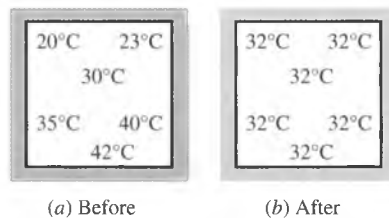
FIGURE 1-28 A closed system reaching thermal equilibrium.
