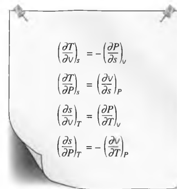
FIGURE 12-8 Maxwell relations are extremely valuable in thermodynamic analysis.
