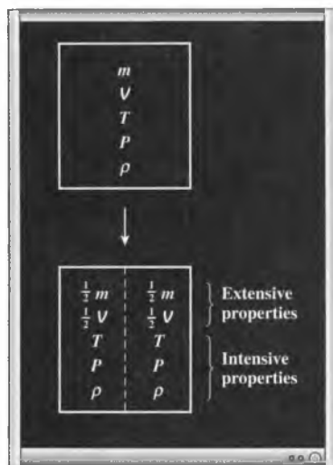
FIGURE 1-24 Criterion to differentiate intensive and extensive properties.
