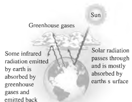
FIGURE 2-68 The greenhouse effect on earth.
