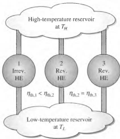
FIGURE 6-40 The Carnot principles.
