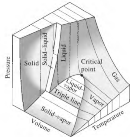
FIGURE 3-24 P - v - T surface of a substance that contracts on freezing.
