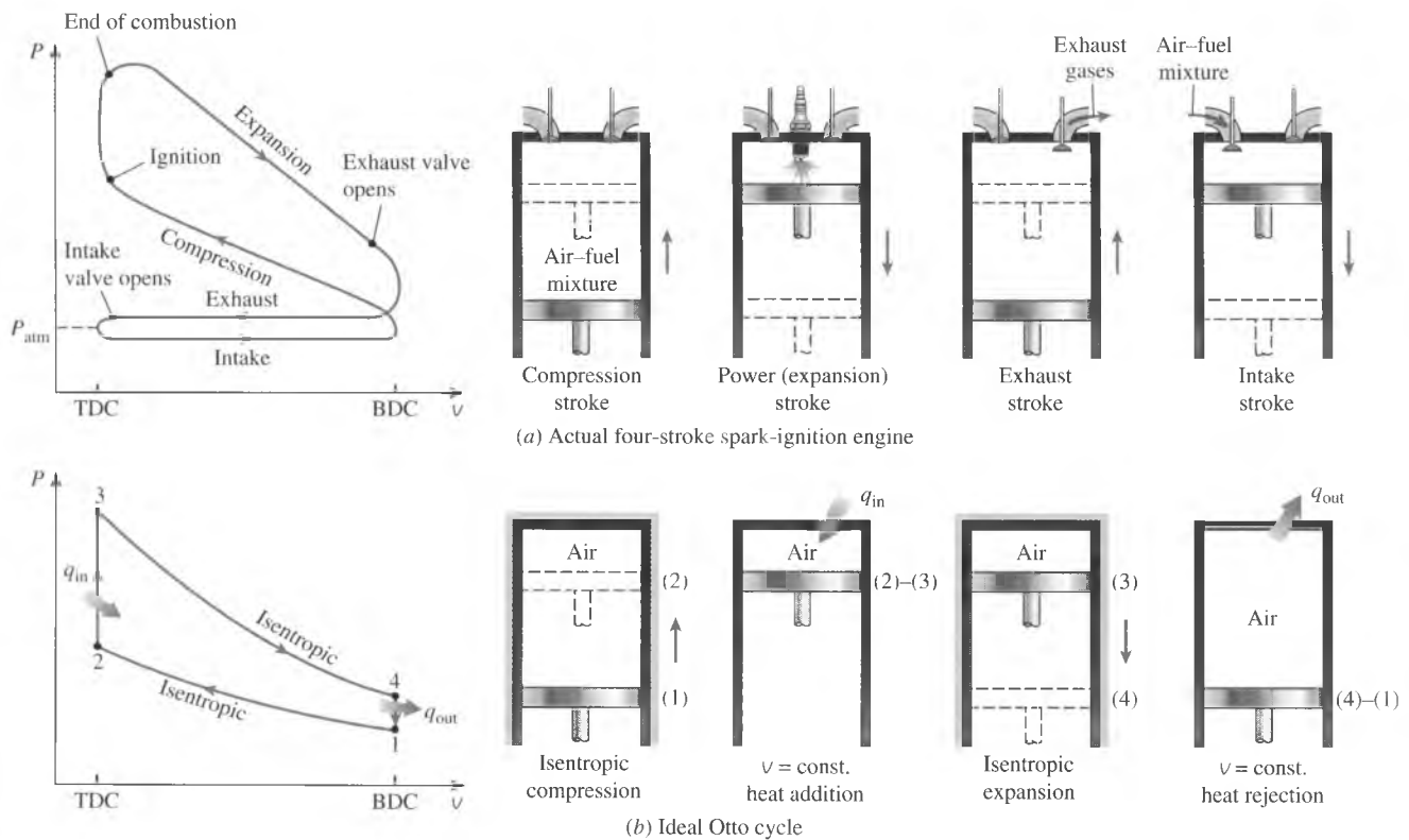
FIGURE 9-13 Actual and ideal cycles in spark-ignition engines and their P - v diagrams.
