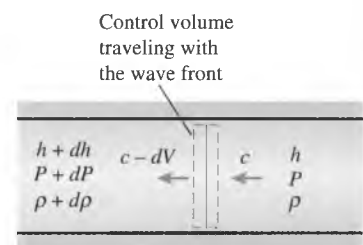
FIGURE 17-8 Control volume moving with the small pressure wave along a duct.
