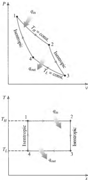
FIGURE 9-6 P - v and T - s diagrams of a Carnot cycle.
