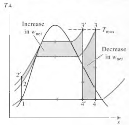
FIGURE 10–8 The effect of increasing the boiler pressure on the ideal Rankine cycle.
