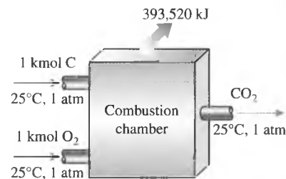
FIGURE 15-16 The formation of \text{CO}_2 during a steady-flow combustion process at 25°C and 1 atm.
