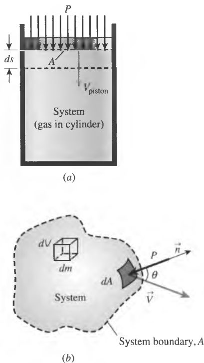
FIGURE 5–50 The pressure force acting on (a) the moving boundary of a system in a piston–cylinder device, and (b) the differential surface area of a system of arbitrary shape.
