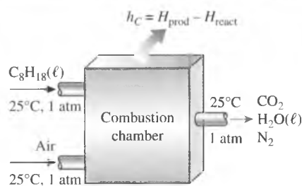
FIGURE 15-20 Schematic for Example 15-5.
