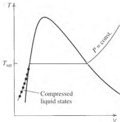
FIGURE 5-34 A substance exists as a compressed liquid at temperatures below the saturation temperatures at the given pressure.
