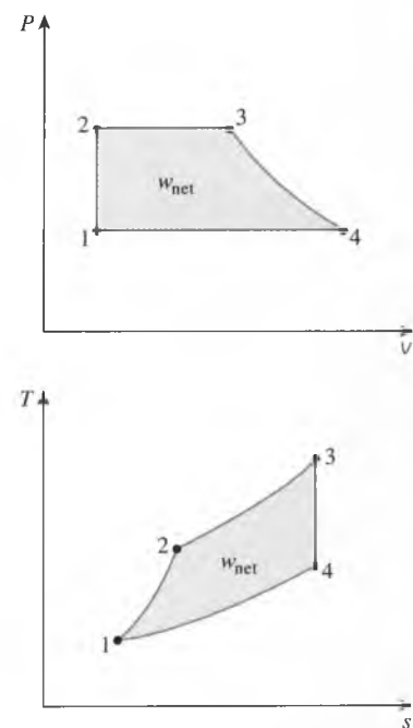
FIGURE 9-5 On both P - v and T - s diagrams, the area enclosed by the process curve represents the net work of the cycle.
