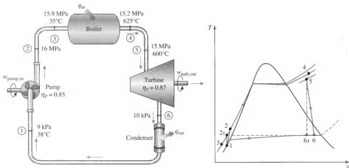
FIGURE 10-5 Schematic and T - s diagram for Example 10-2.
