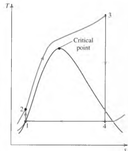
FIGURE 10–9 A supercritical Rankine cycle.
