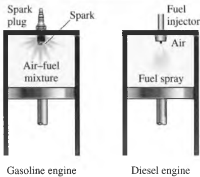
FIGURE 9-20 In diesel engines, the spark plug is replaced by a fuel injector, and only air is compressed during the compression process.
