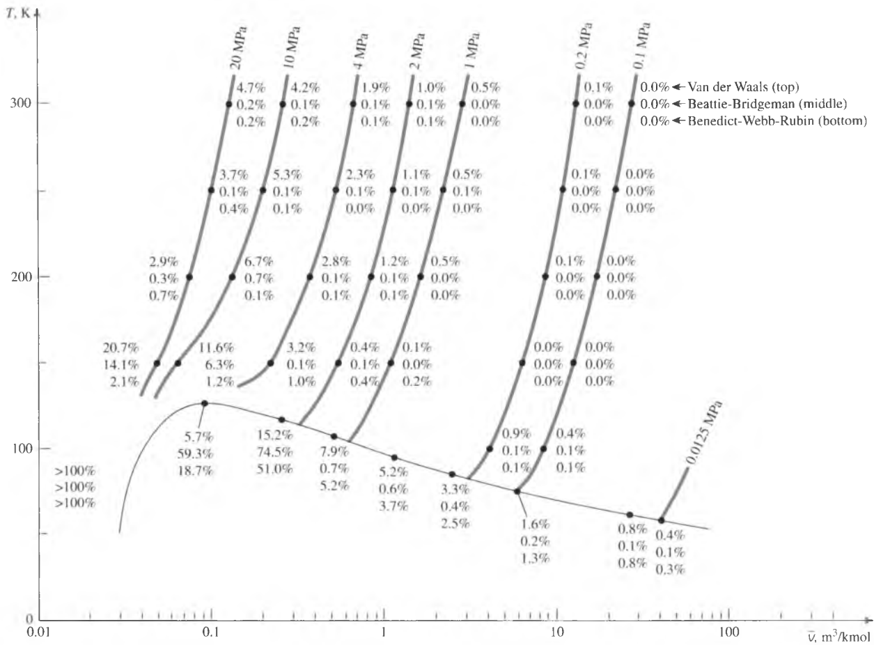
FIGURE 3-58 Percentage of error involved in various equations of state for nitrogen ( \% \text{ error} = [(v_{\text{table}} - v_{\text{equation}})/v_{\text{table}}] \times 100 ).
