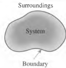
FIGURE 1–19 System, surroundings, and boundary.
