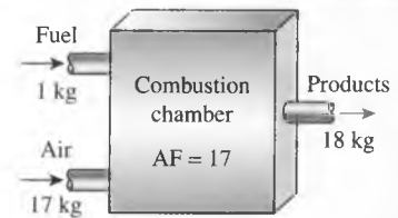
FIGURE 15–6 The air–fuel ratio (AF) represents the amount of air used per unit mass of fuel during a combustion process.
