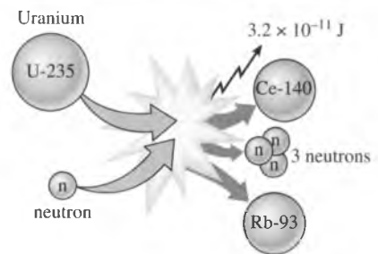
(a) Fission of uranium
