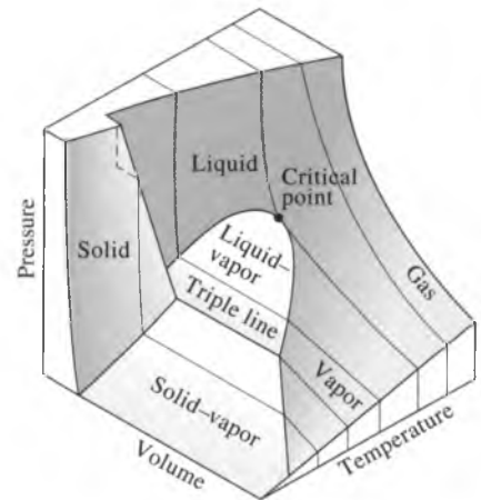
FIGURE 3-25 P - v - T surface of a substance that expands on freezing (like water).
