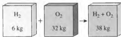
FIGURE 13-1 The mass of a mixture is equal to the sum of the masses of its components.
