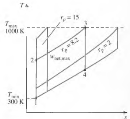
FIGURE 9–33 For fixed values of T_{\min} and T_{\max} , the net work of the Brayton cycle first increases with the pressure ratio, then reaches a maximum at r_p = (T_{\max}/T_{\min})^{k/[2(k-1)]} , and finally decreases.
