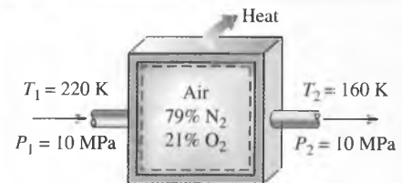
FIGURE 13-17 Schematic for Example 13-5.
