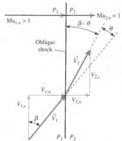
FIGURE 17-41 The same velocity vectors of Fig. 17-40, but rotated by angle \pi/2 - \beta , so that the oblique shock is vertical. Normal Mach numbers Ma_{1,n} and Ma_{2,n} are also defined.
