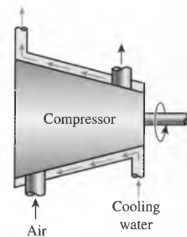
FIGURE 7-52 Compressors are sometimes intentionally cooled to minimize the work input.
