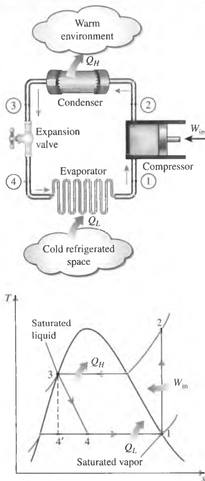
FIGURE 11-3 Schematic and T - s diagram for the ideal vapor-compression refrigeration cycle.
