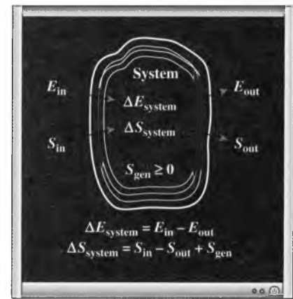
FIGURE 7-57 Energy and entropy balances for a system.
