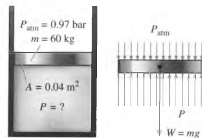
FIGURE 1–58 Schematic for Example 1–9; and the free-body diagram of the piston.
