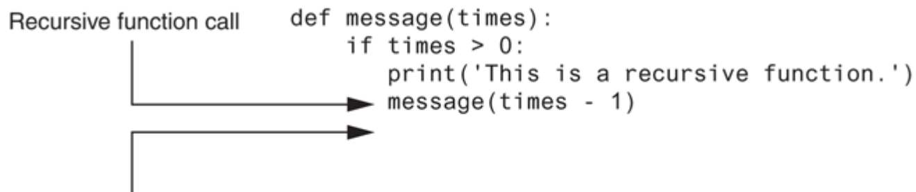
Figure 12-3 Control returns to the point after the recursive function call
