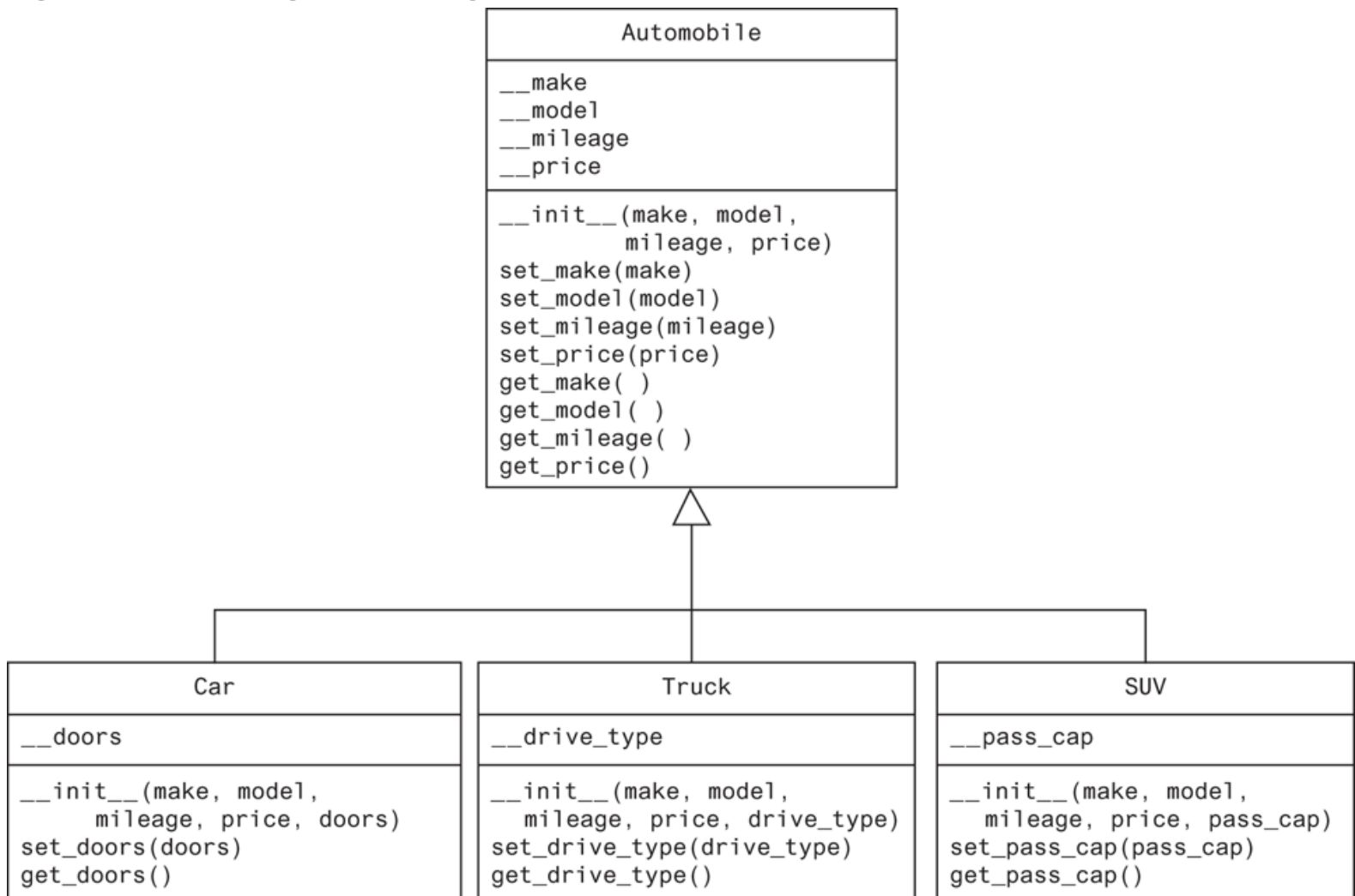
Figure 11-2 UML diagram showing inheritance
