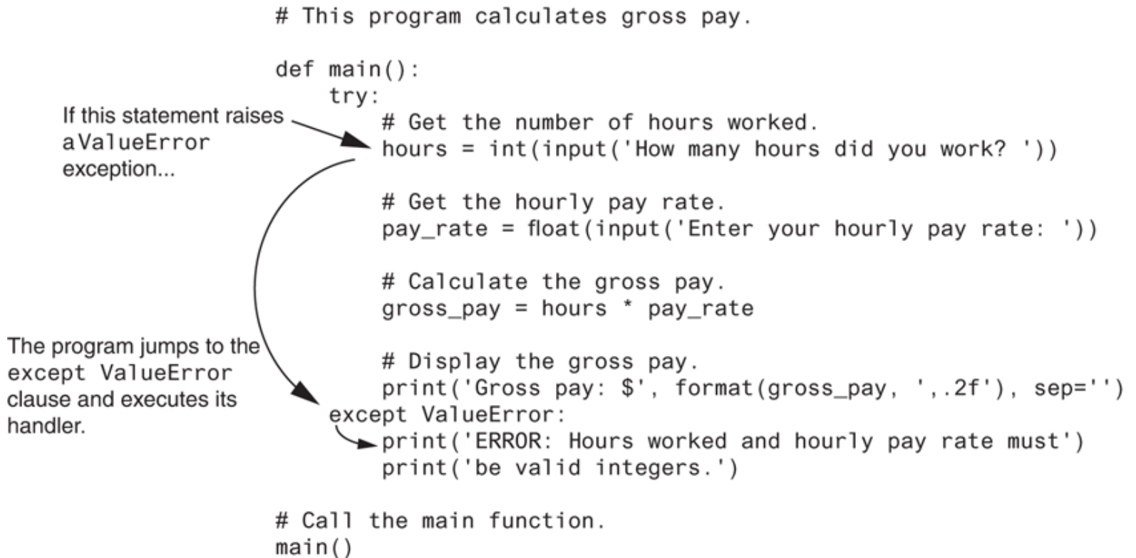
Figure 6-20 Handling an exception
