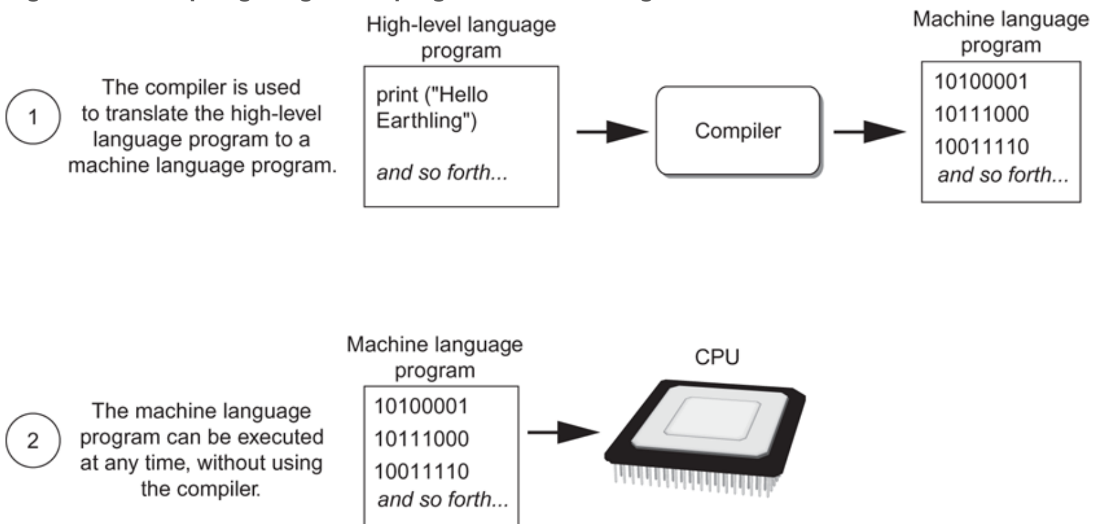
Figure 1-18 Compiling a high-level program and executing it
