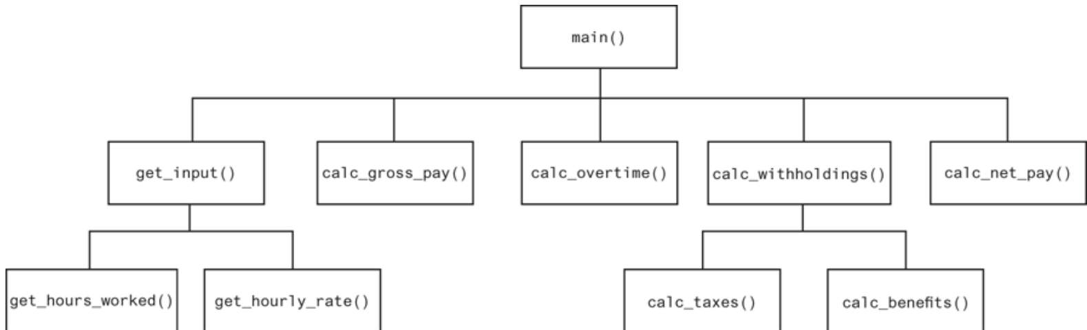
Figure 5-10 A hierarchy chart
