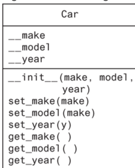
Figure 10-14 UML diagram for the Car class
