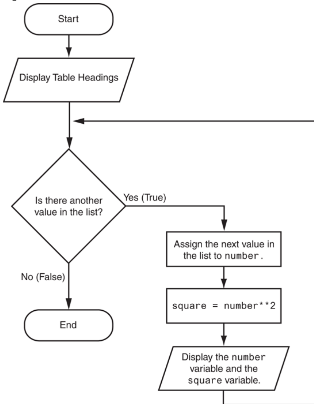
Figure 4-5 Flowchart for Program 4-8
