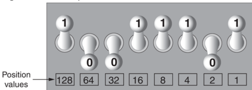
Figure 1-11 The bit pattern for 157
