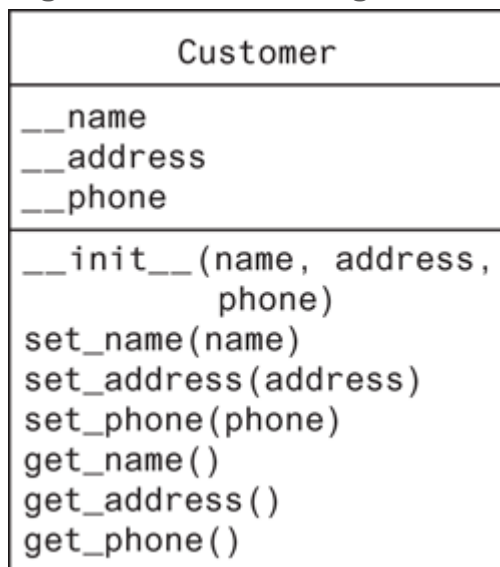
Figure 10-13 UML diagram for the Customer class
