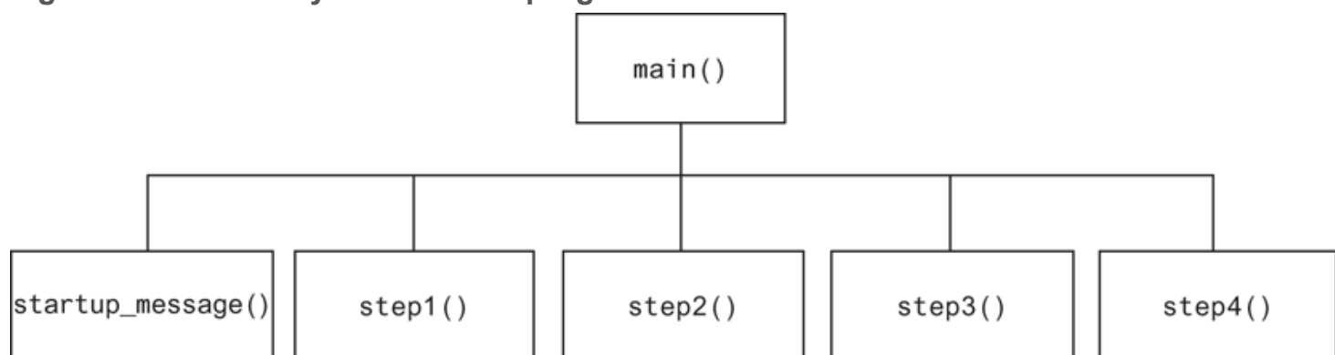
Figure 5-11 Hierarchy chart for the program
