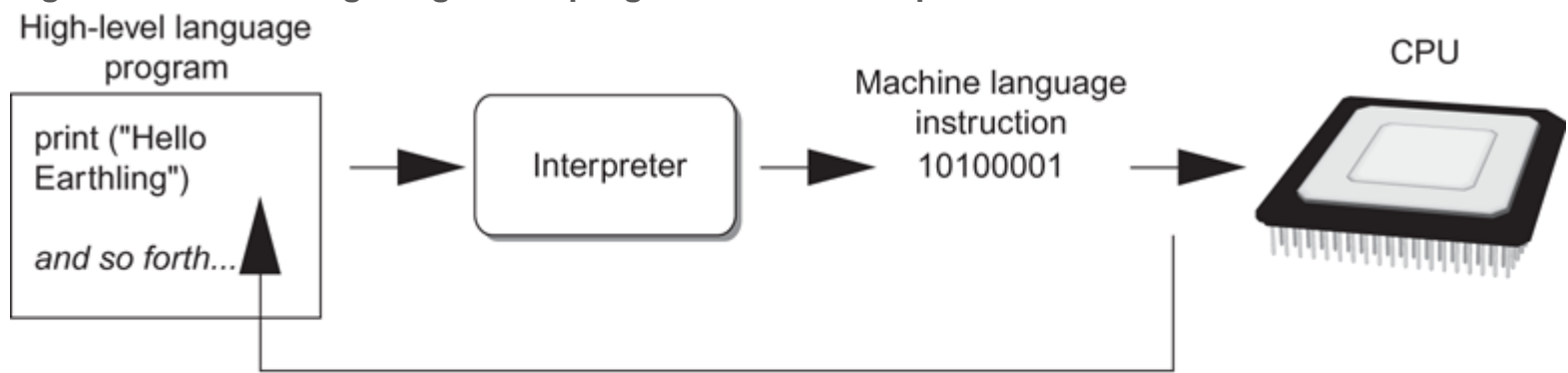
Figure 1-19 Executing a high-level program with an interpreter
