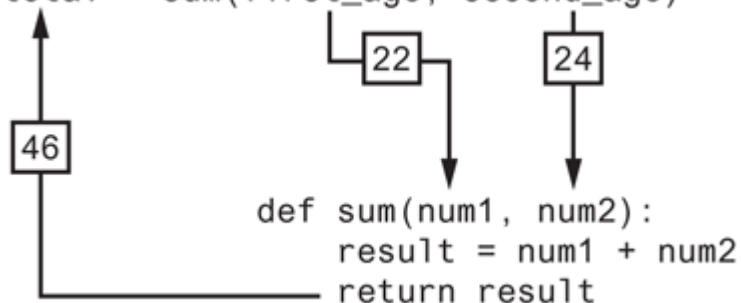
Figure 5-24 Arguments are passed to the sum function and a value is returned
