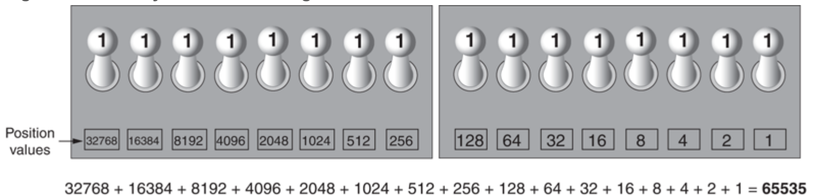
Figure 1-12 Two bytes used for a large number
