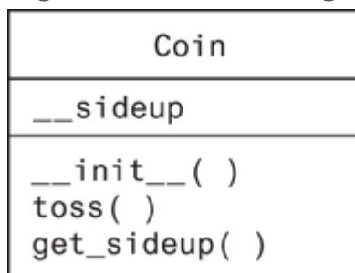
Figure 10-11 UML diagram for the Coin class
