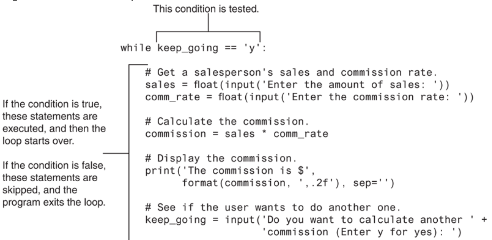
Figure 4-2 The while loop
