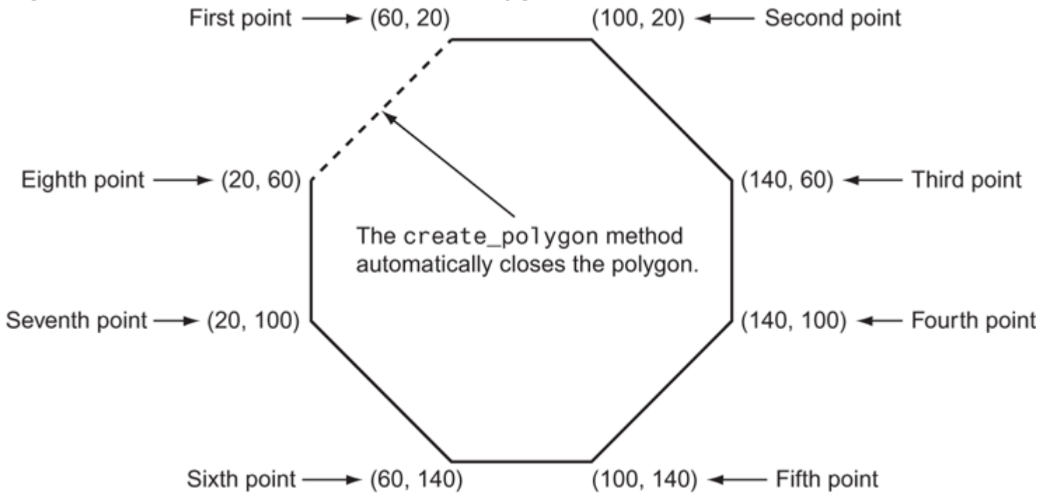
Figure 13-37 Points of each vertex in the polygon
