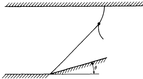
Figure 4.28 | Mach reflection.
