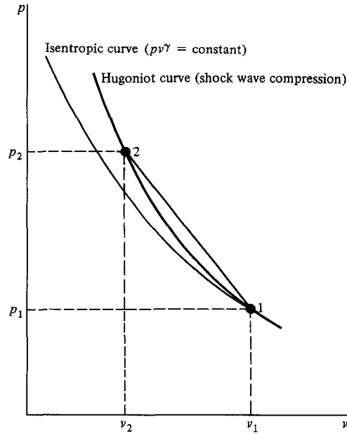
Figure 3.11 | Hugoniot curve; comparison with isentropic compression.
