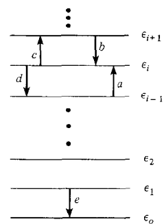
Figure 16.16 | Single quantum transitions for vibrational energy exchange.
