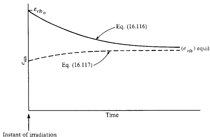
Figure 16.17 | Vibrational relaxation toward equilibrium.
