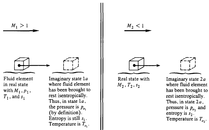
Figure 3.9 | Illustration of total (stagnation) conditions ahead of and behind a normal shock wave.
