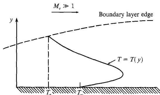
Figure 15.5 | Schematic of a temperature profile in a hypersonic boundary layer.
