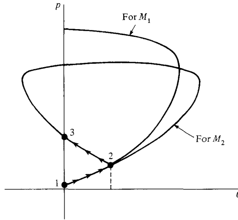
Figure 4.22 | The reflected shock process on a pressure-deflection diagram.
