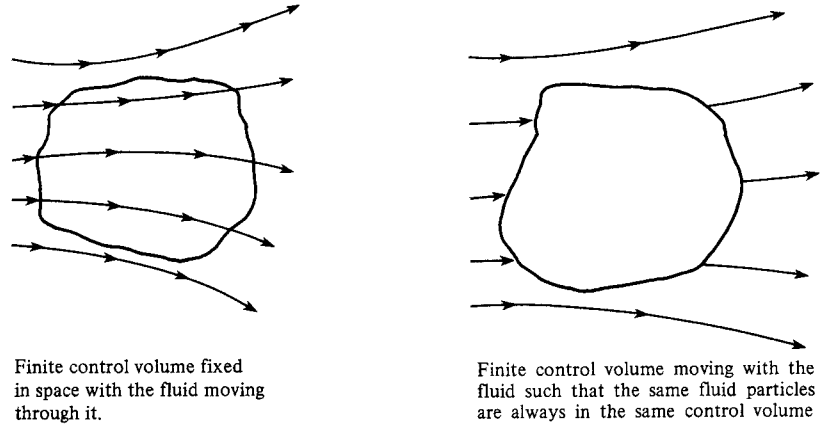
Figure 2.2 | Finite control volume approach.
