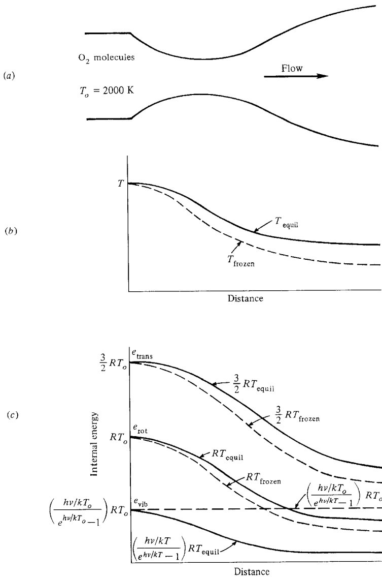
Figure 17.9 | A schematic comparing equilibrium and frozen vibrationally relaxing flows through a nozzle.
