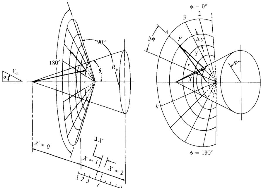
Figure 13.15 | Coordinate system and finite-difference mesh for the calculations of Ref. 90.
