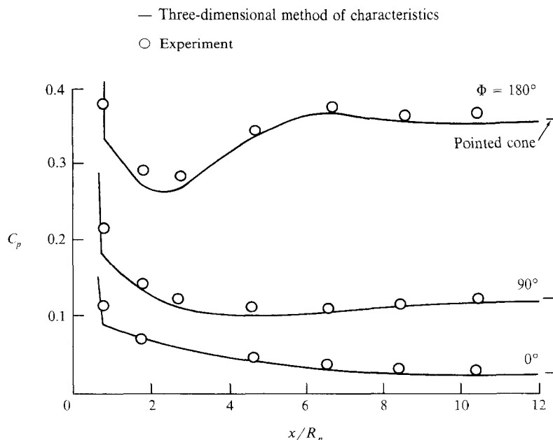
Figure 15.16 | Pressure distributions over a blunt-nosed cone; comparison between theory and experiment in air. \alpha = 10^\circ , Re = 0.6 \times 10^6 , M_\infty = 10 , \gamma = 1.4 . (From Ref. 129.)
